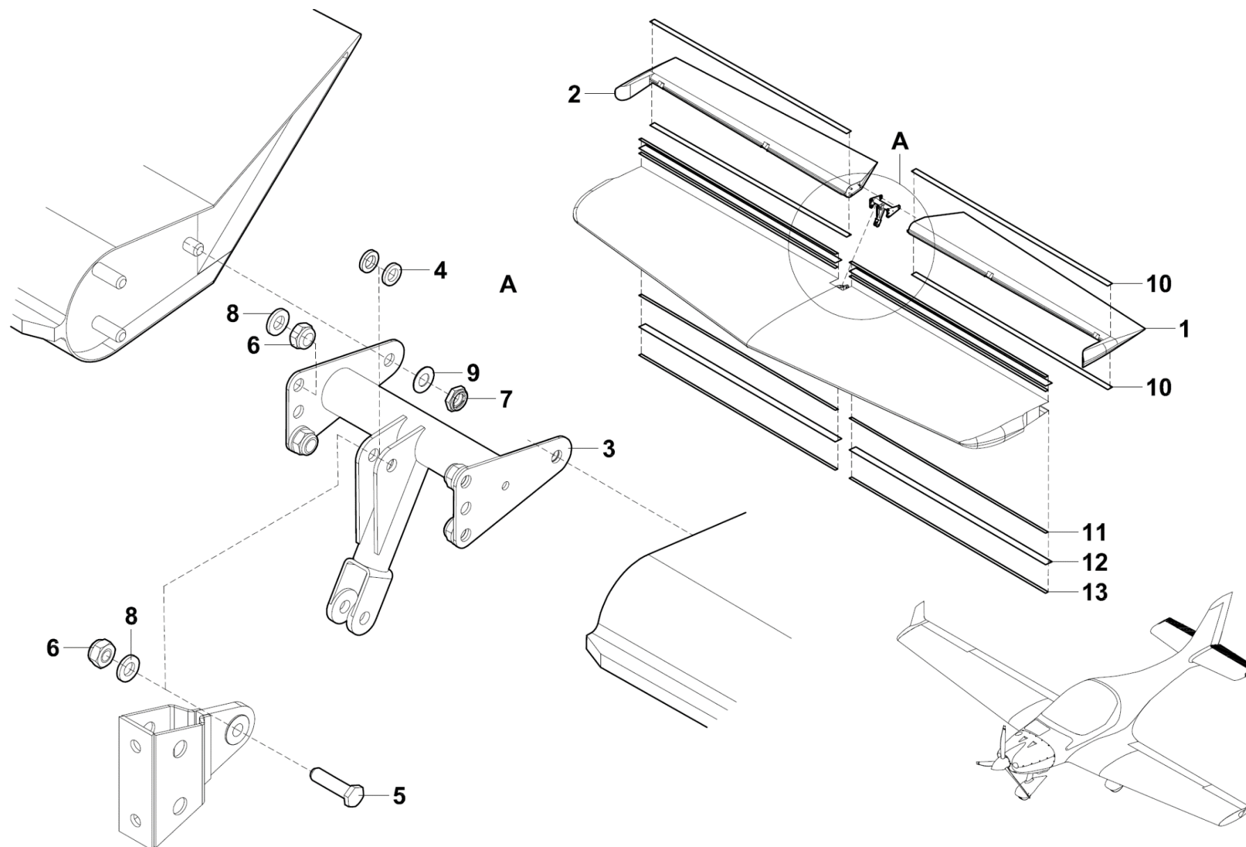
55-20-01 Elevator LSA
