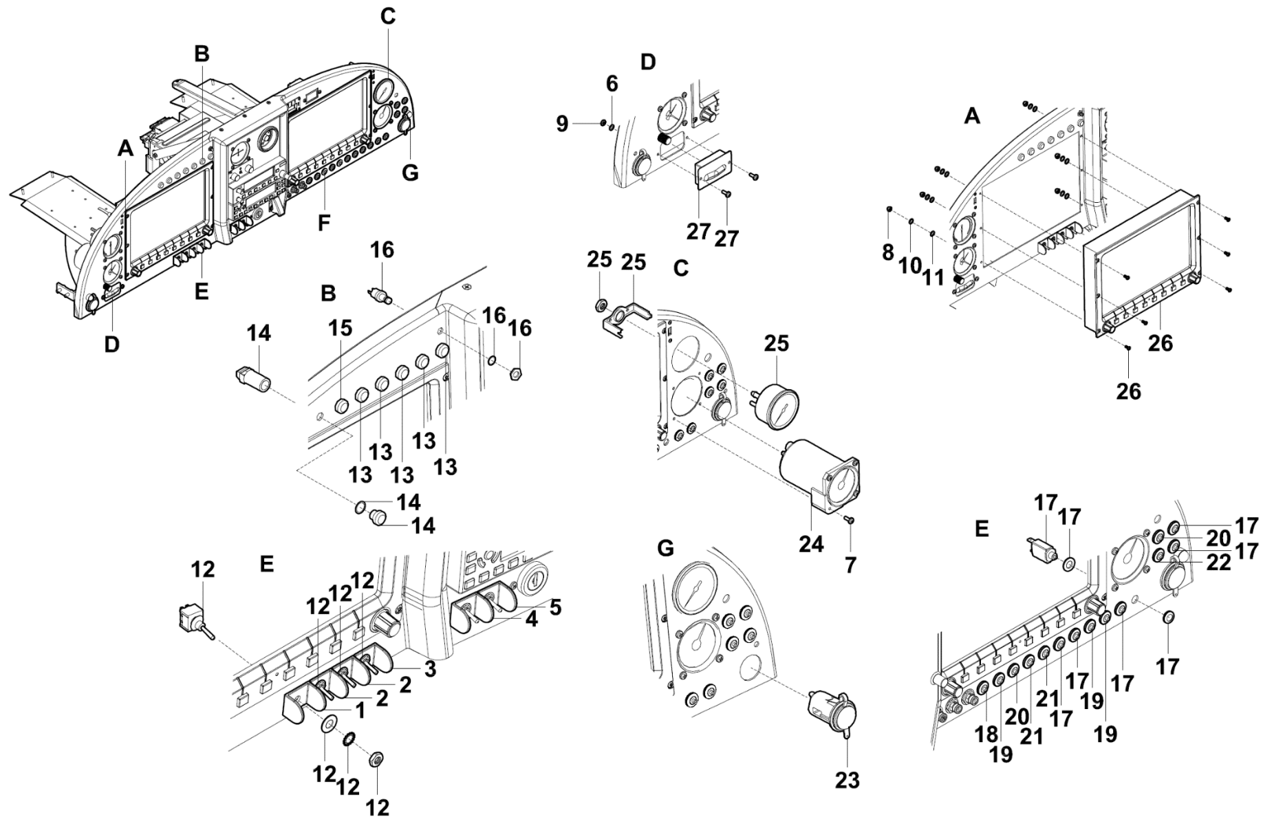
Figure 39-10-04 Instrument Panel Installation
