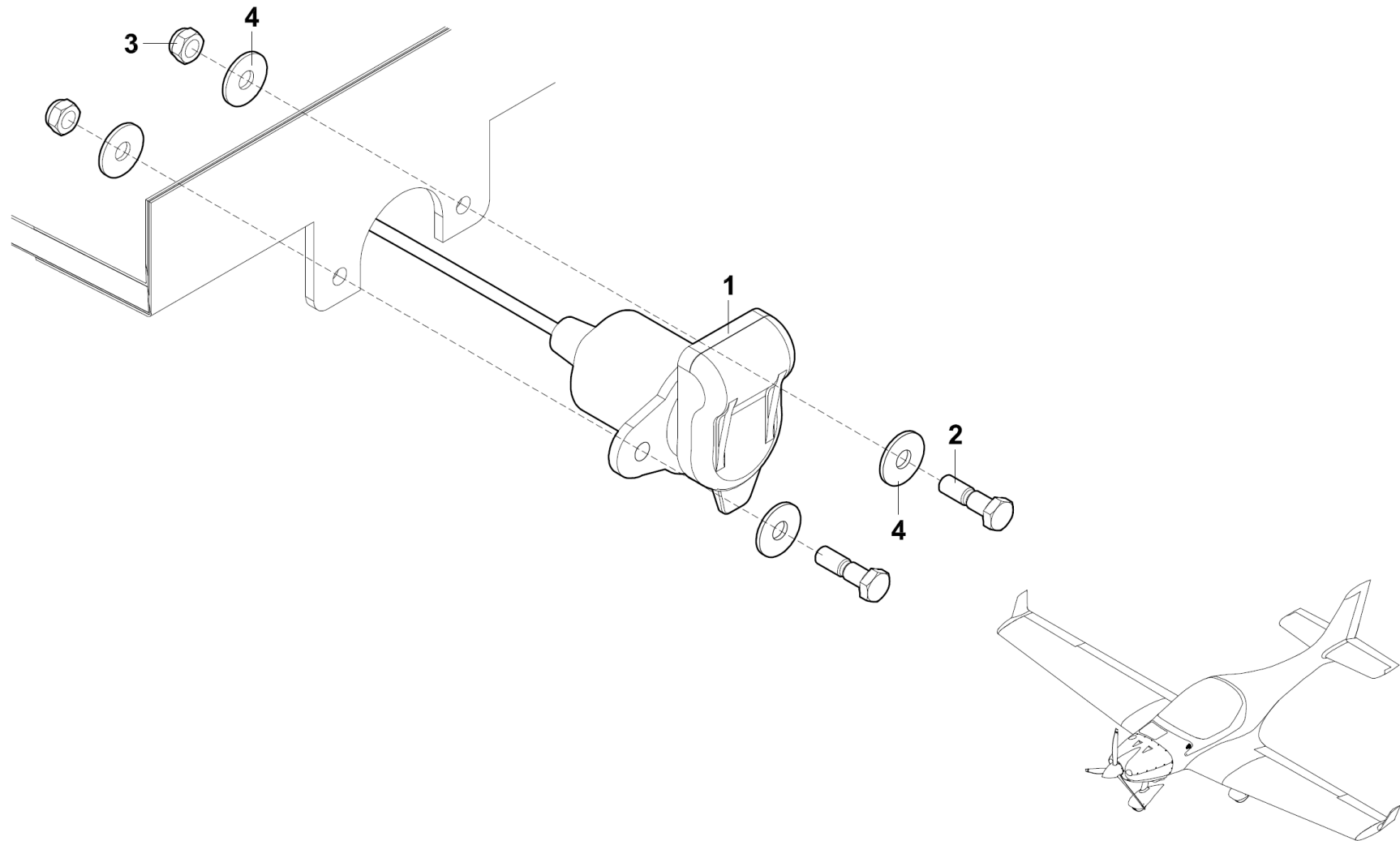
Figure 24-40 External power LSA
