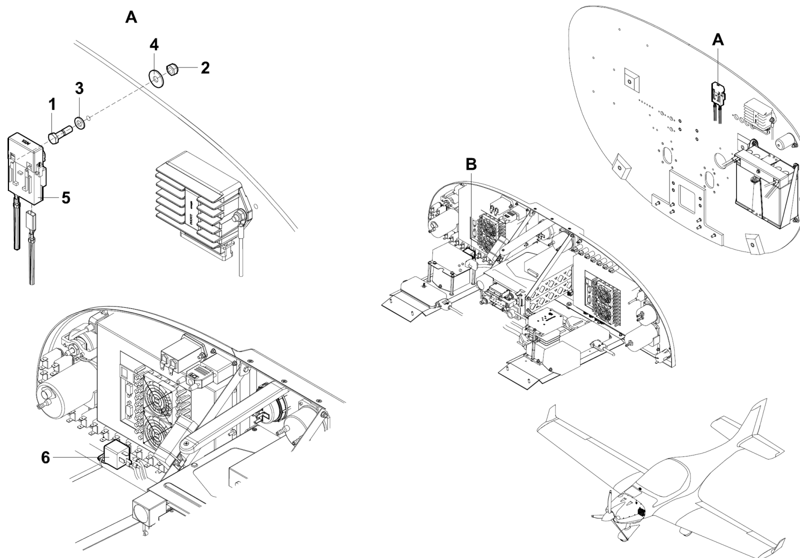
Figure 24-60-01 DC Distribution LSA
