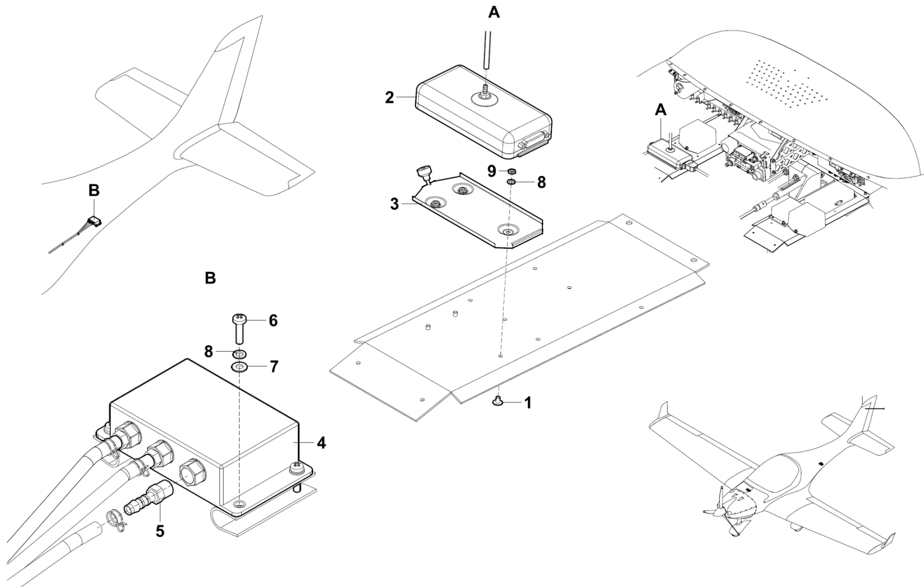
Figure 34-10-03 Flight Environment Data
