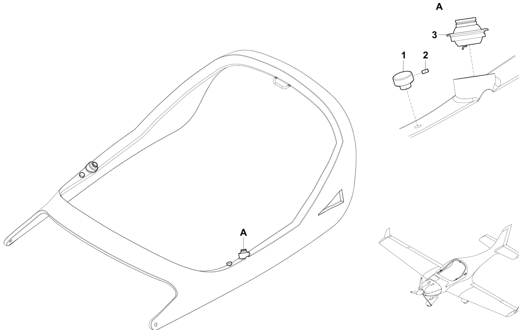
Figure 21-20-02 Venting LSA
