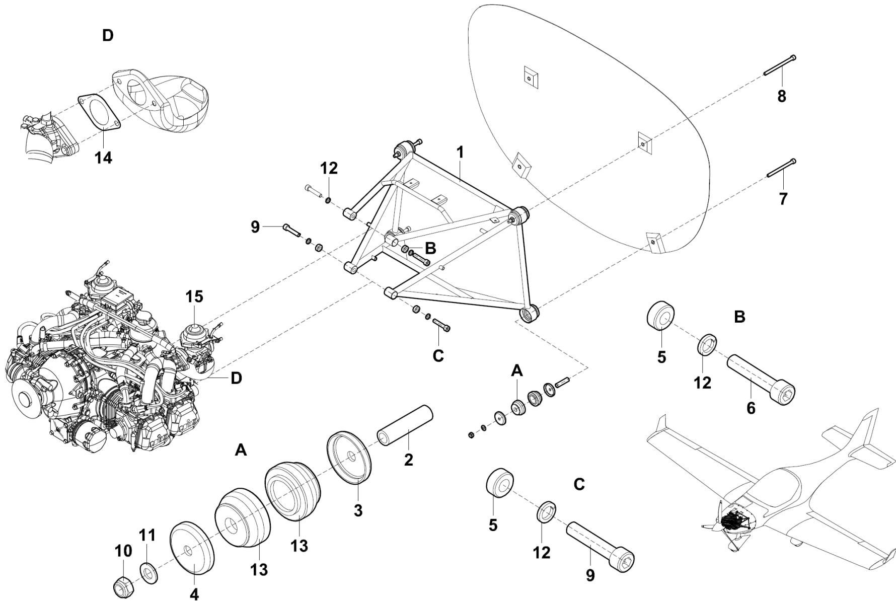
Figure 71-20-01 Engine attachment LSA
