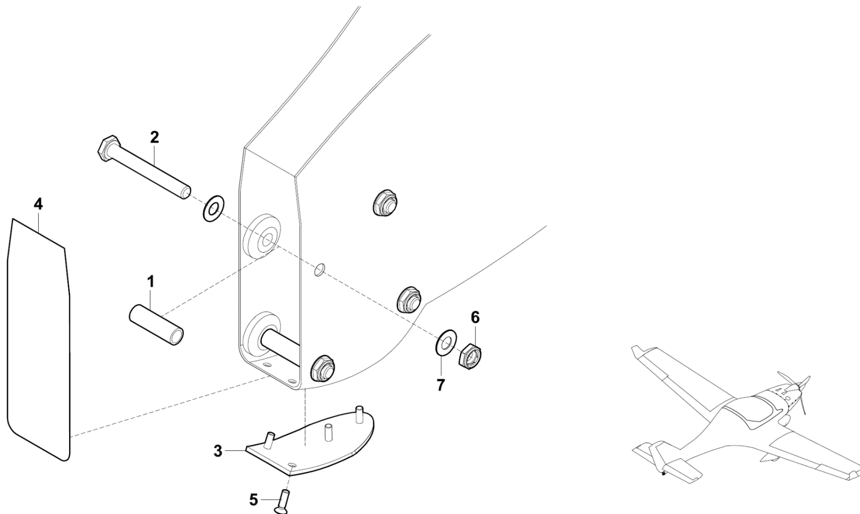
Figure 95-10-01 Towing equipment preparation
