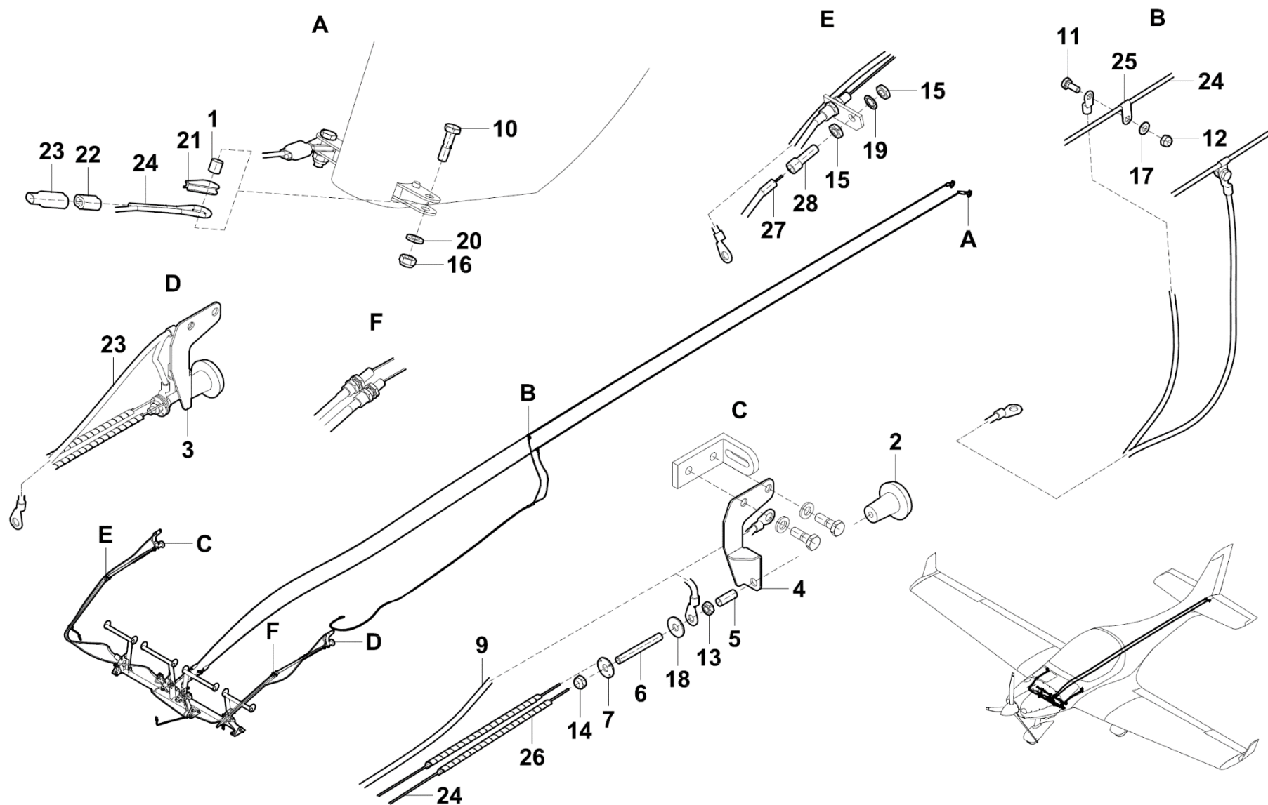
Figure 27-20-01 Rudder Control LSA
