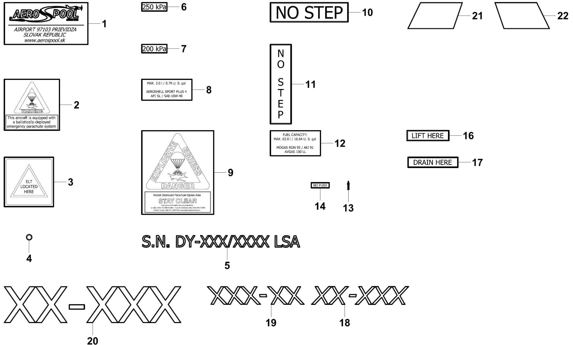
Figure 11-20-02 Placards and labels, Exterior
