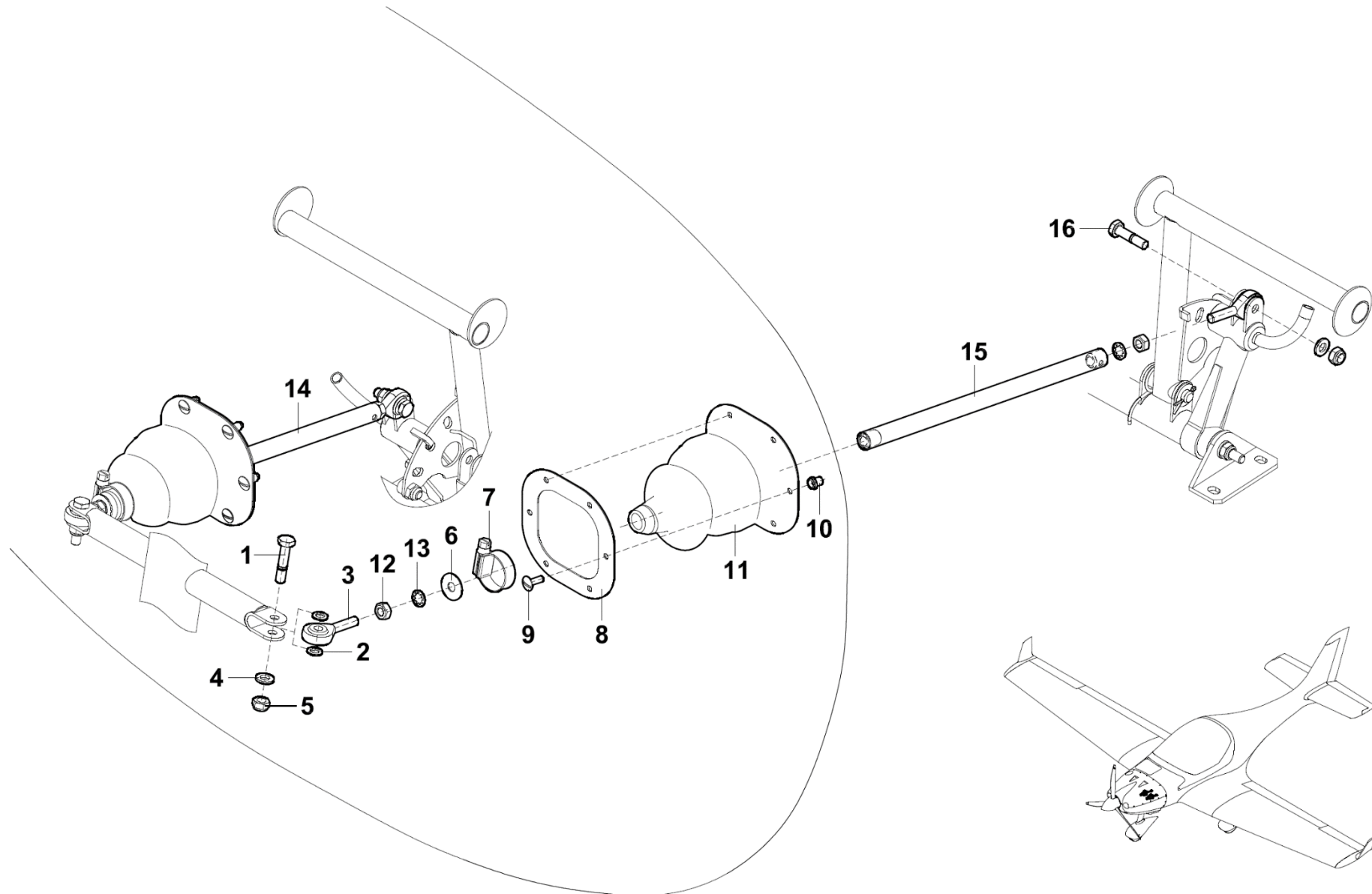
Figure 32-50 Nose Gear Steering
