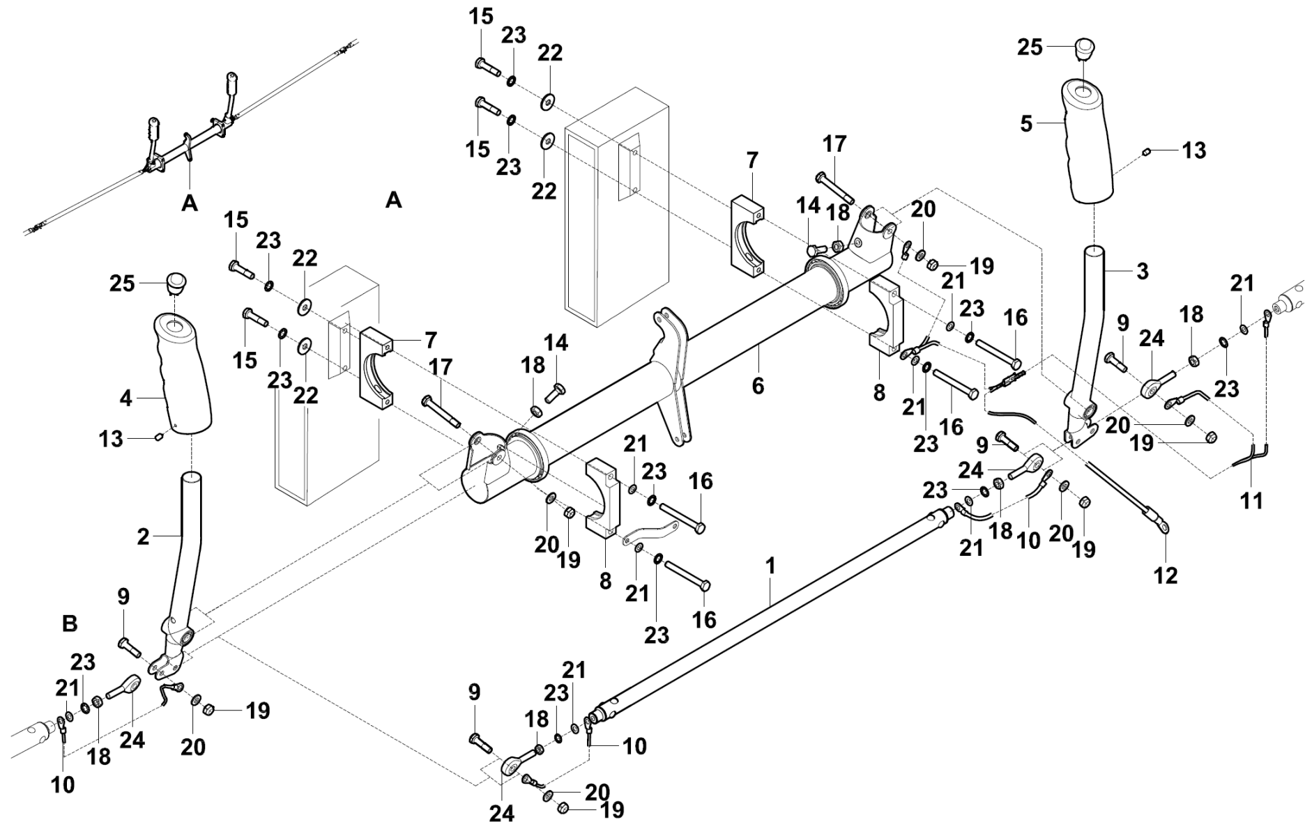
Figure 27-10-02 Aileron Control LSA
