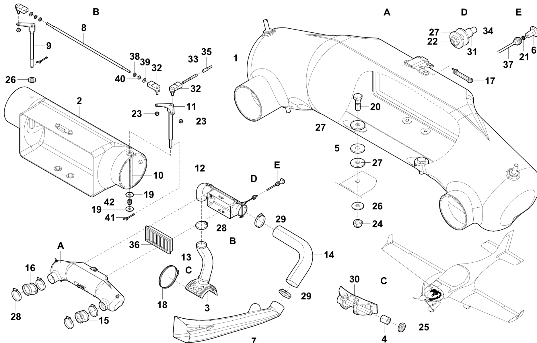
Figure 71-60-01 Engine intake LSA
