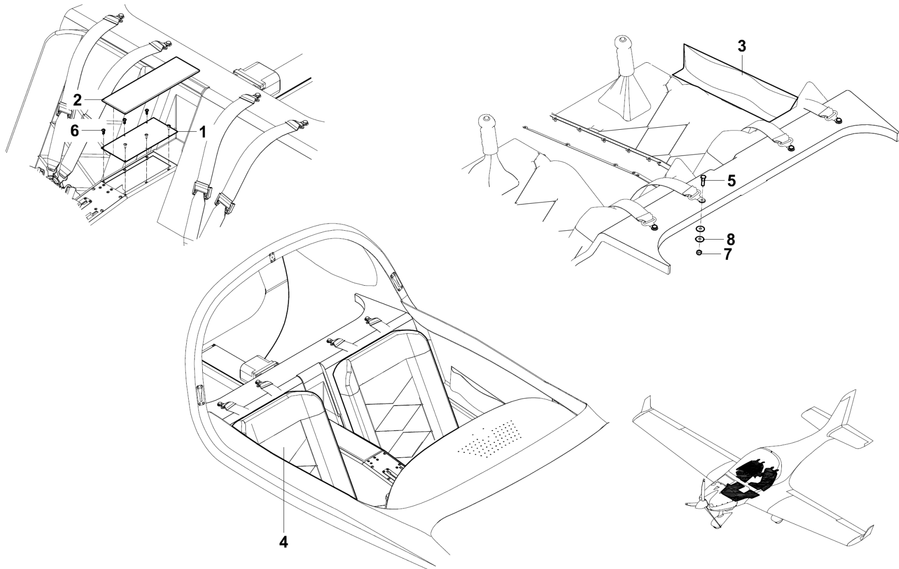
Figure 25-10-01 Flight compartment LSA
