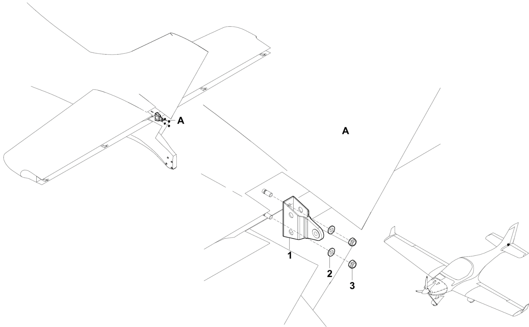
Figure 55-10-01 Horizontal stabilizer
