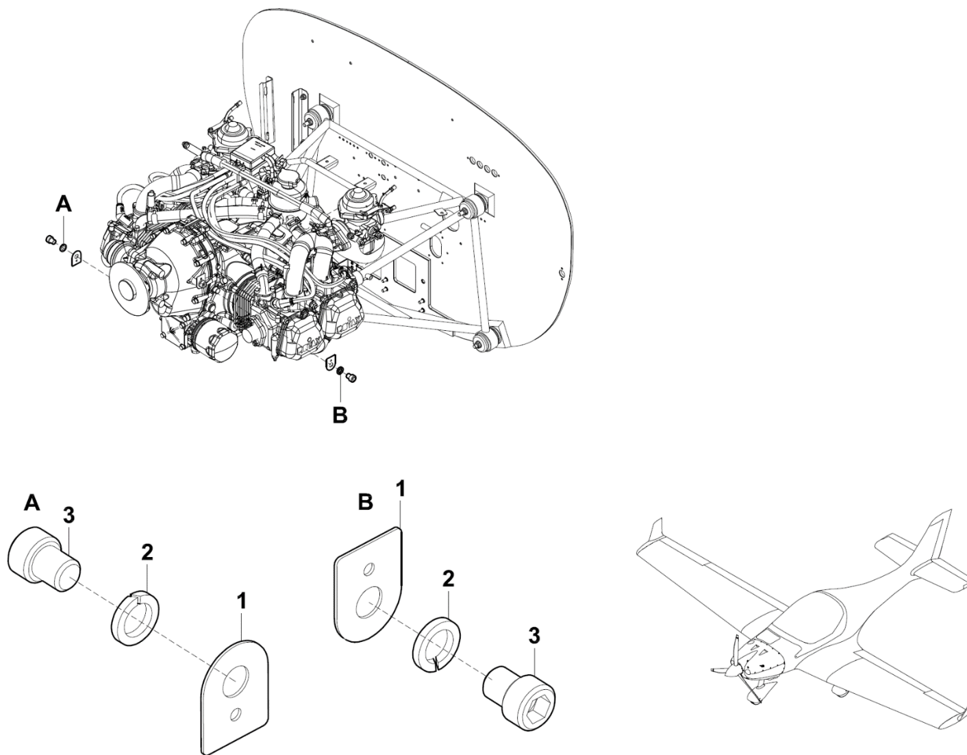
Figure 71-40-01 Engine compartment holder
