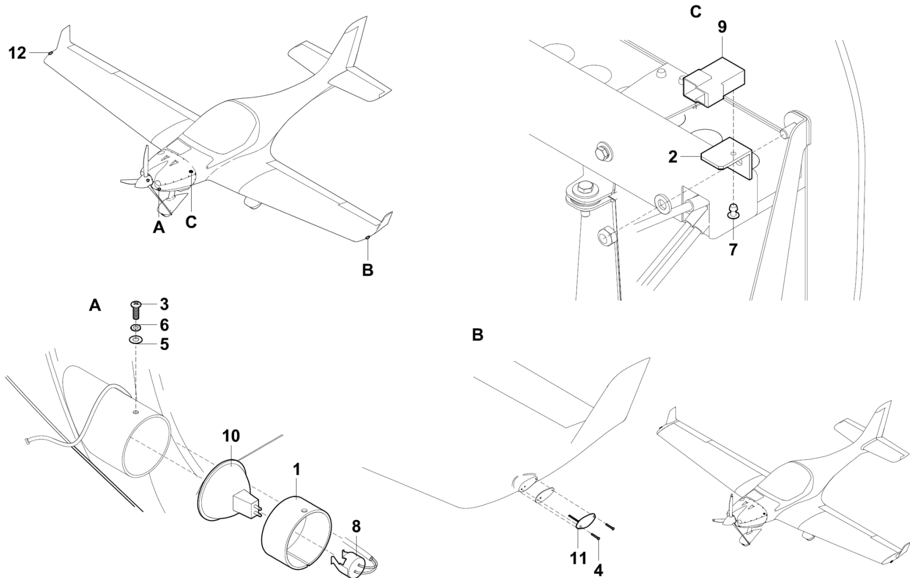
Figure 33-40-01 Exterior lighting LSA
