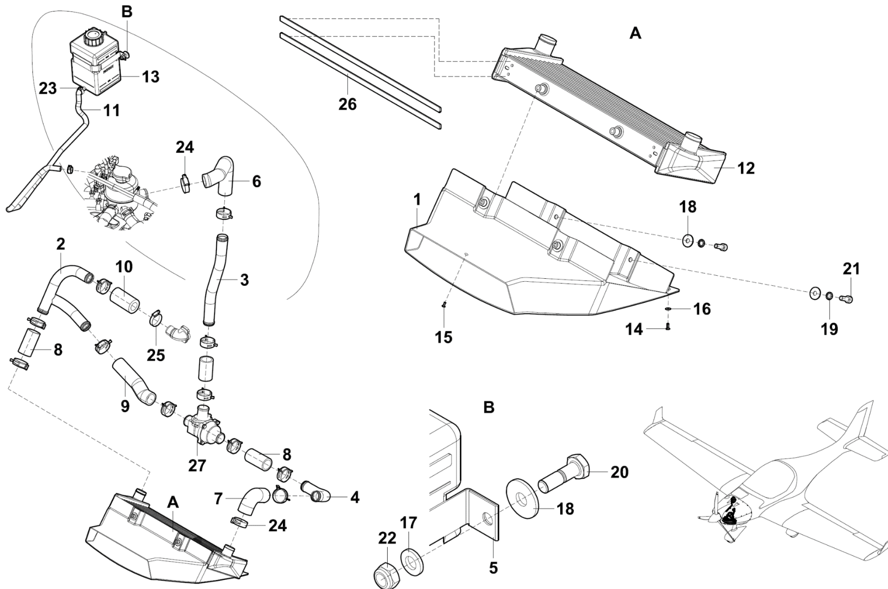
Figure 75-20-01 Engine cooling
