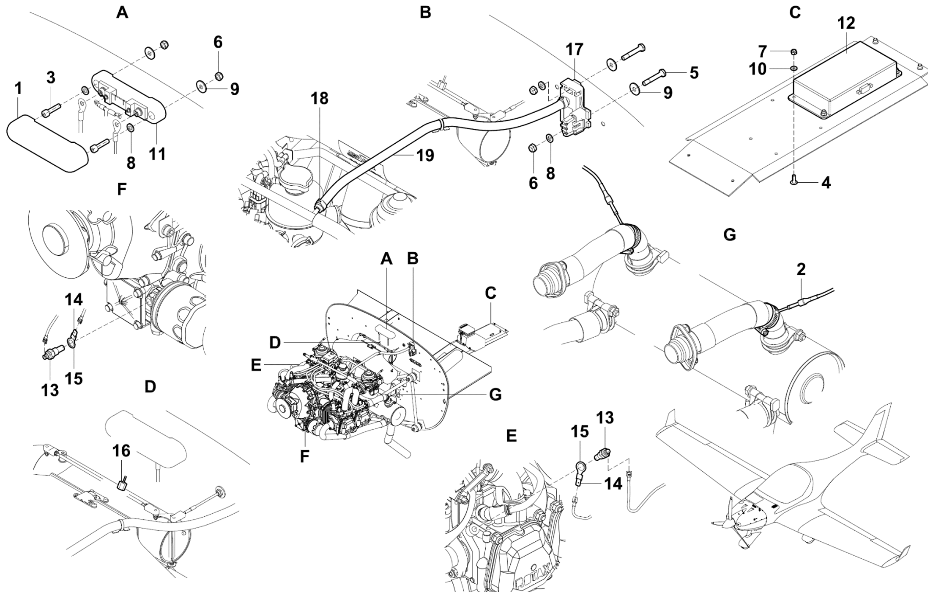
Figure 77-40-01 Engine Sensors LSA
