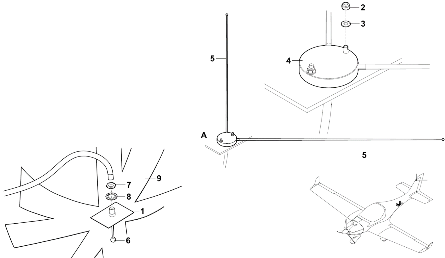
Figure 34-50-01 Dependent position determining
