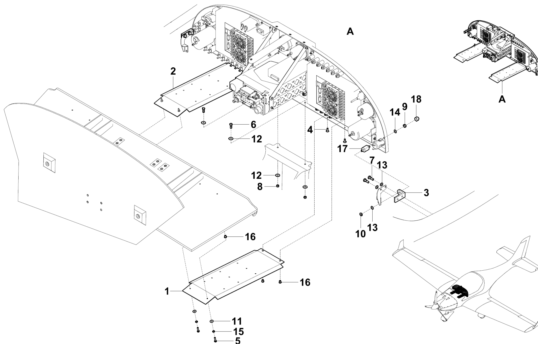
Figure 39-10-01 Instrument Panel Installation
