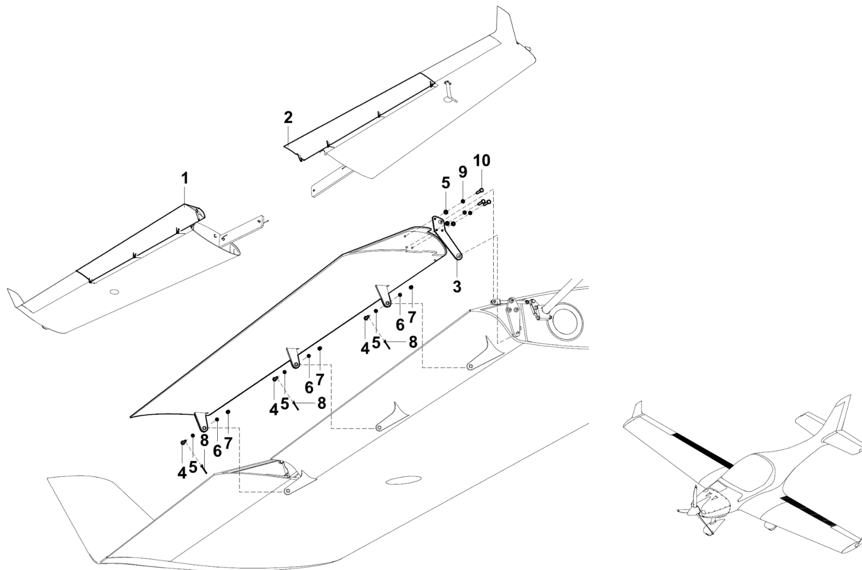
Figure 57-50 Flaps LSA
