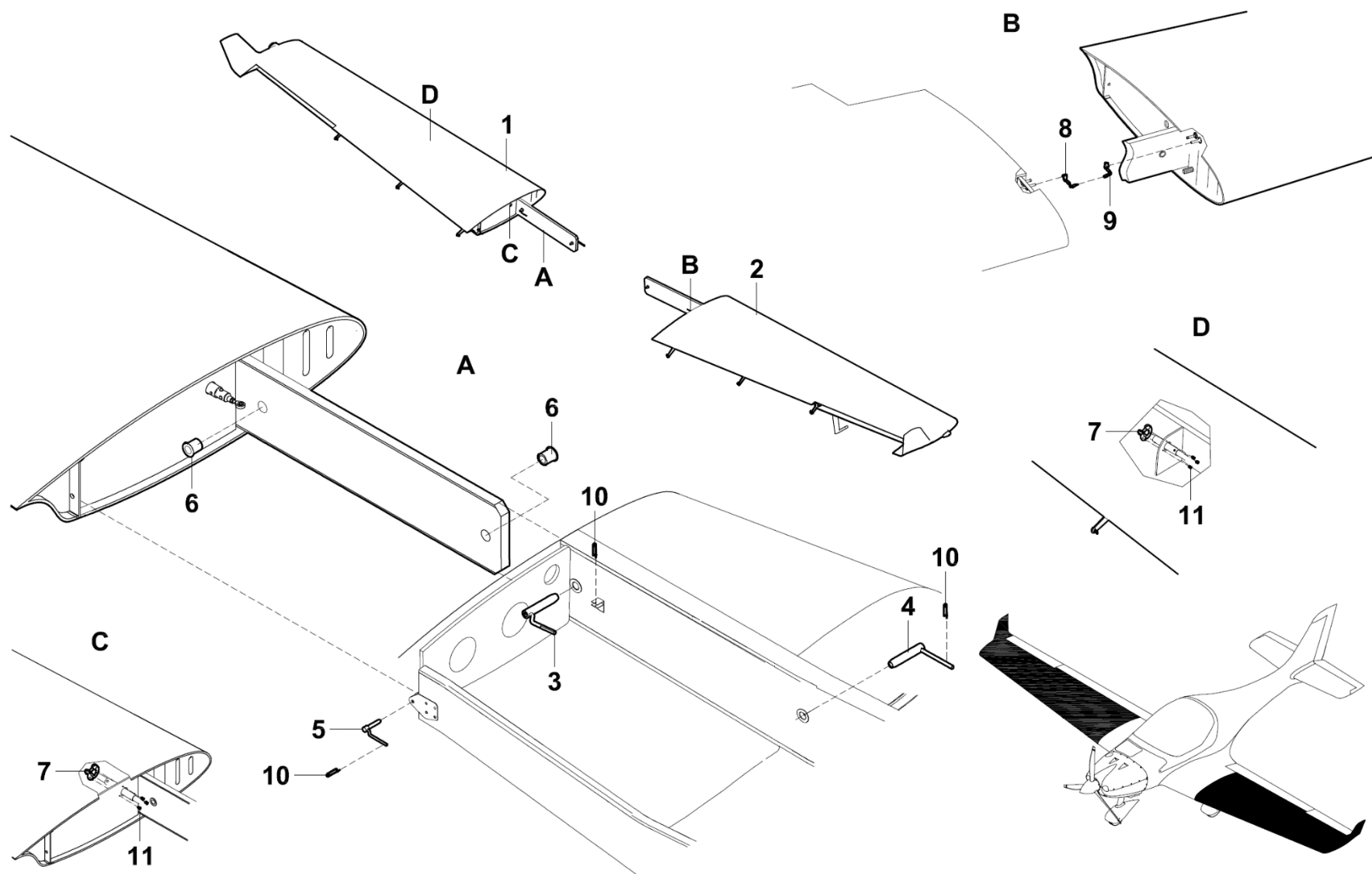
Figure 57-20 Wings LSA
