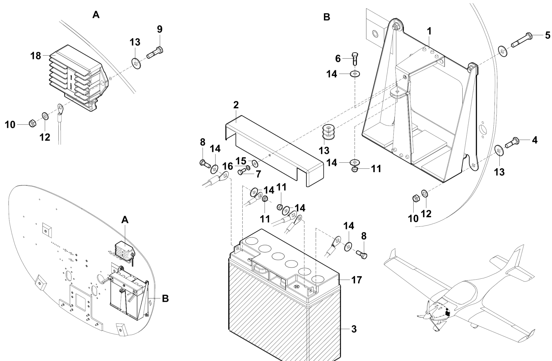
Figure 24-30-01 DC Generation LSA
