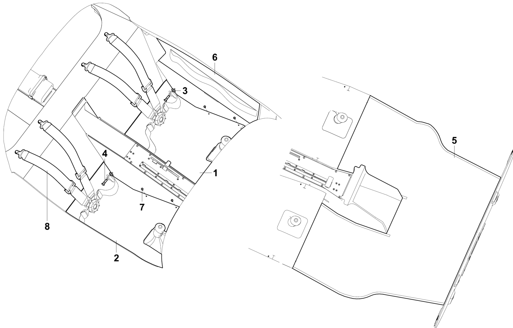
Figure 25-10-02 Flight compartment LSA
