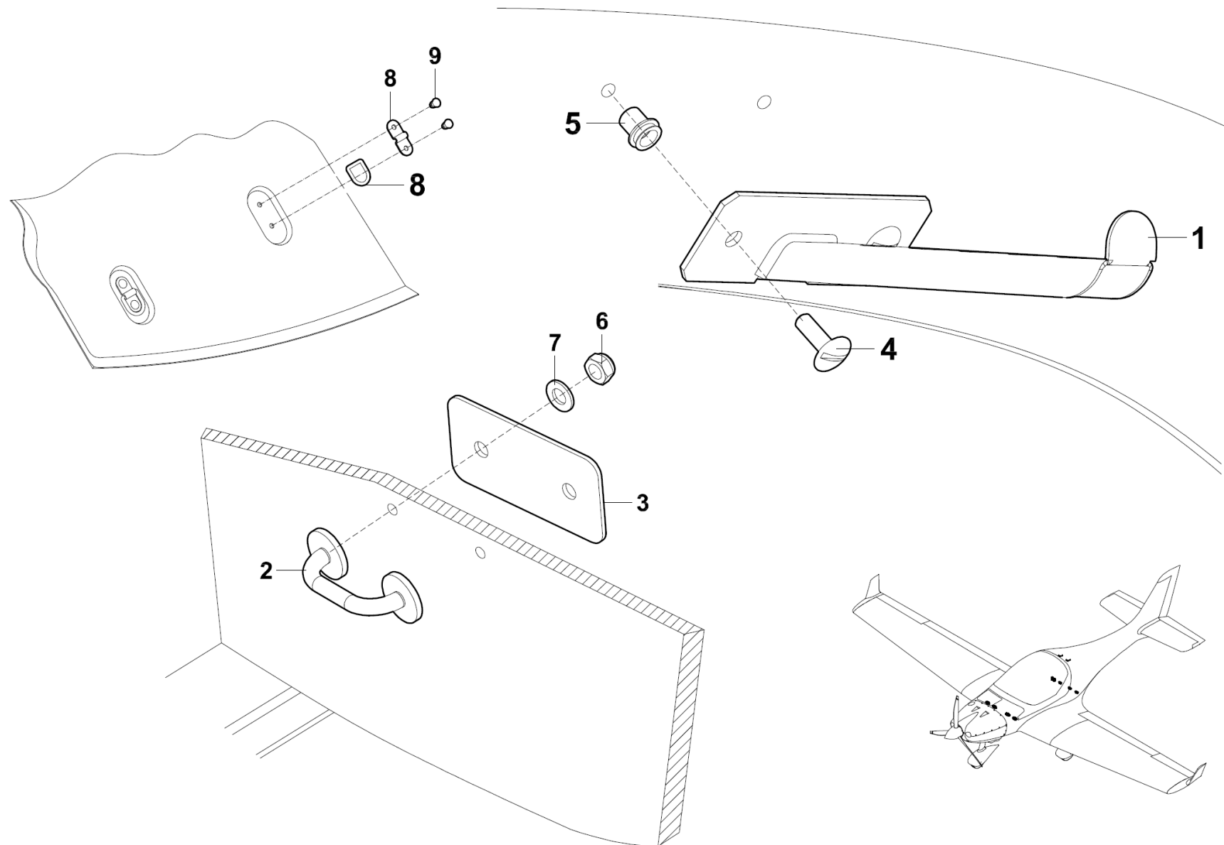
Figure 25-50 Baggage compartment LSA
