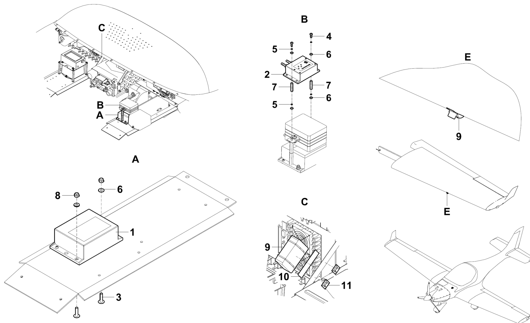
Figure 31-50-01 Central Warning Systems
