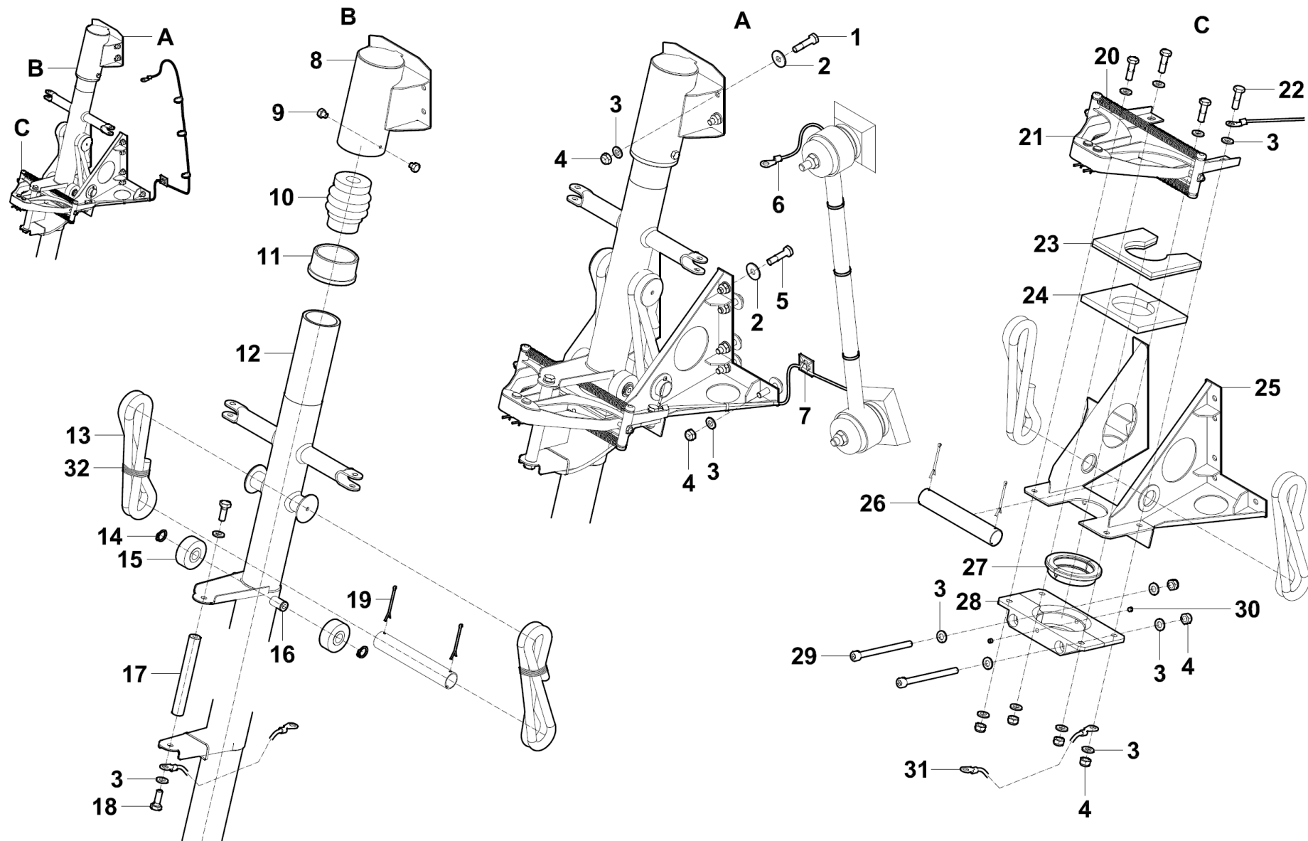
Figure 32-20-02 Nose Gear LSA
