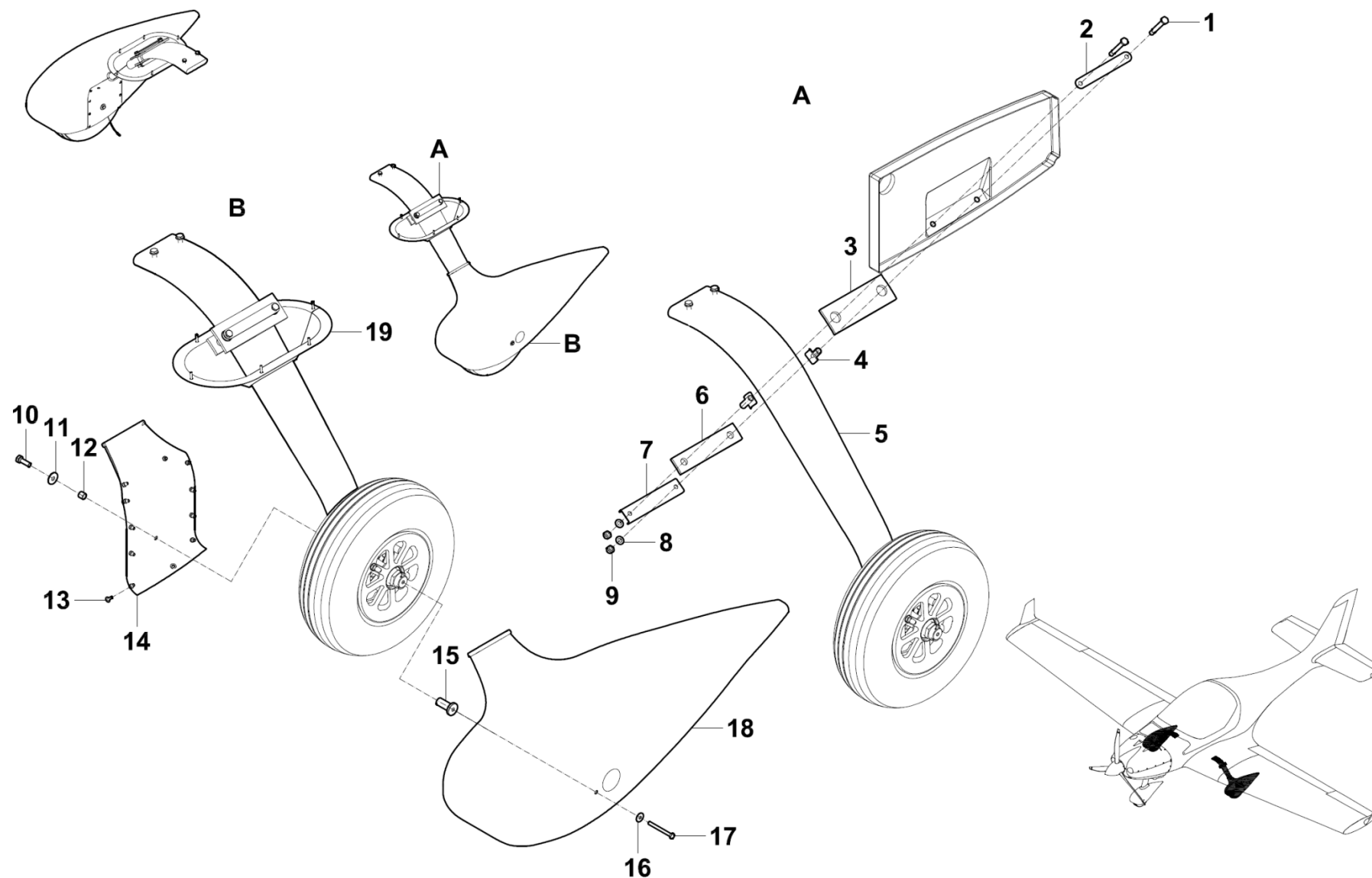
Figure 32-10-01 Main Gear LSA
