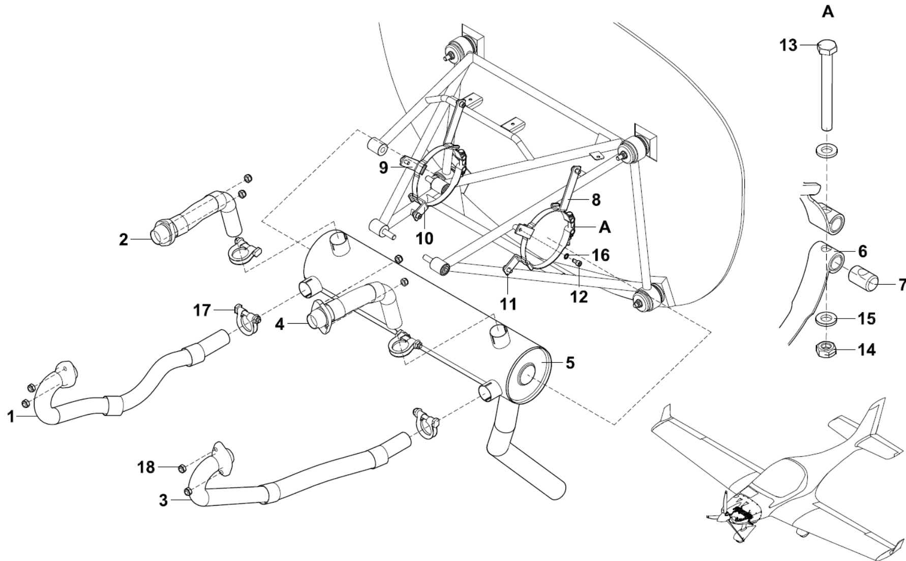
Figure 78-10-01 Exhaust system LSA
