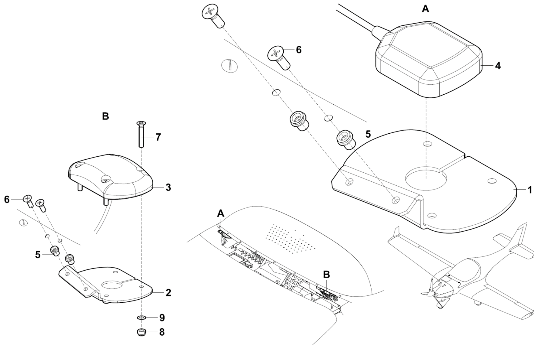
Figure 34-50-02 Dependent position determining
