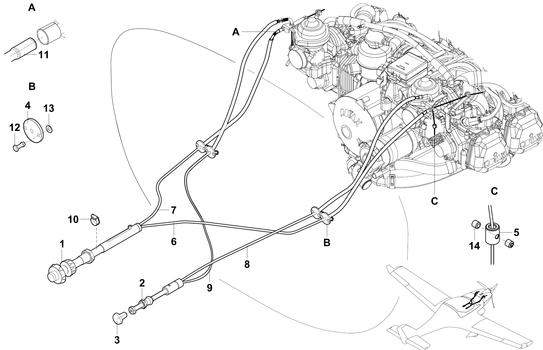
Figure 76-10-01 Engine Controllers
