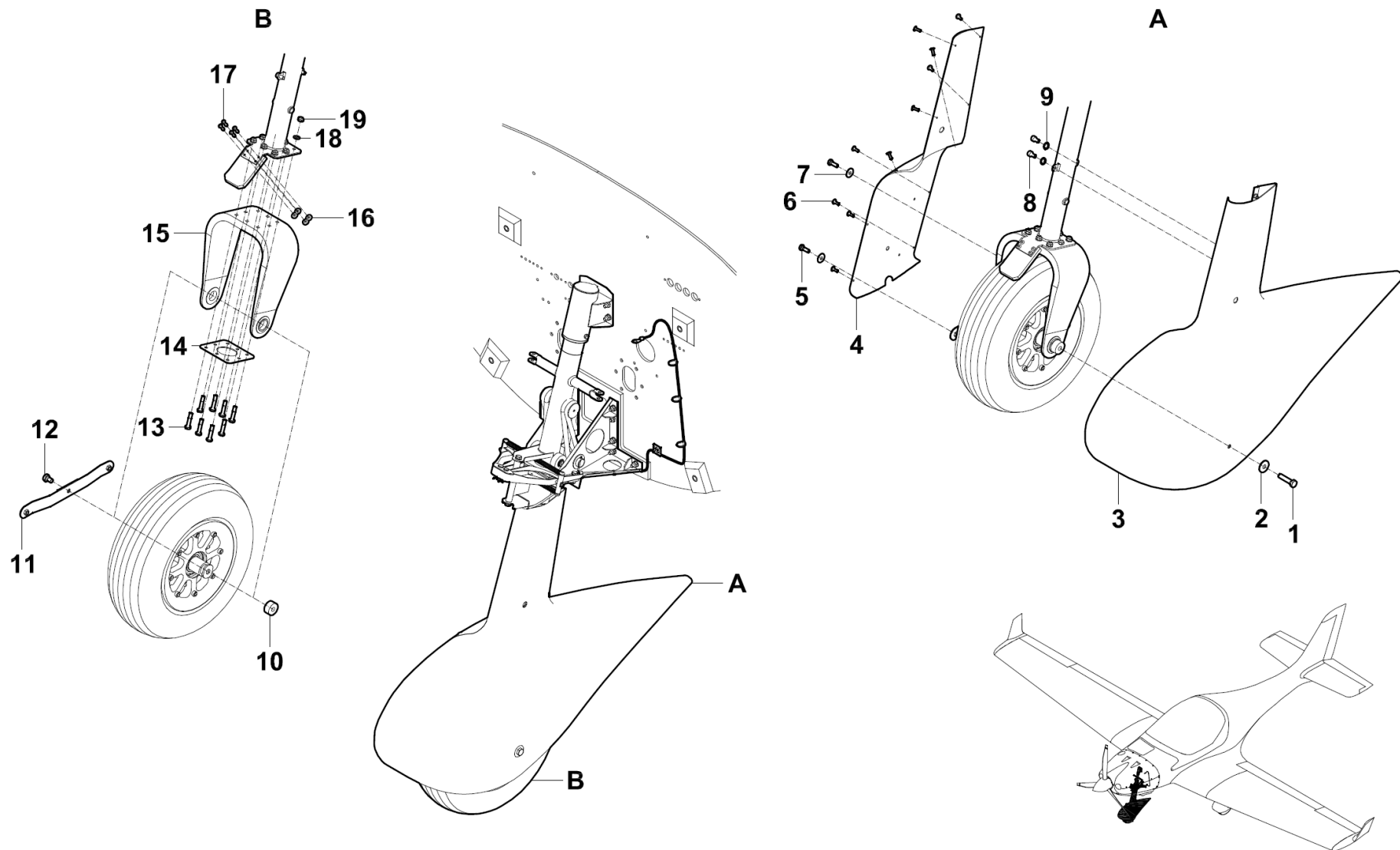
Figure 32-20-01 Nose Gear LSA
