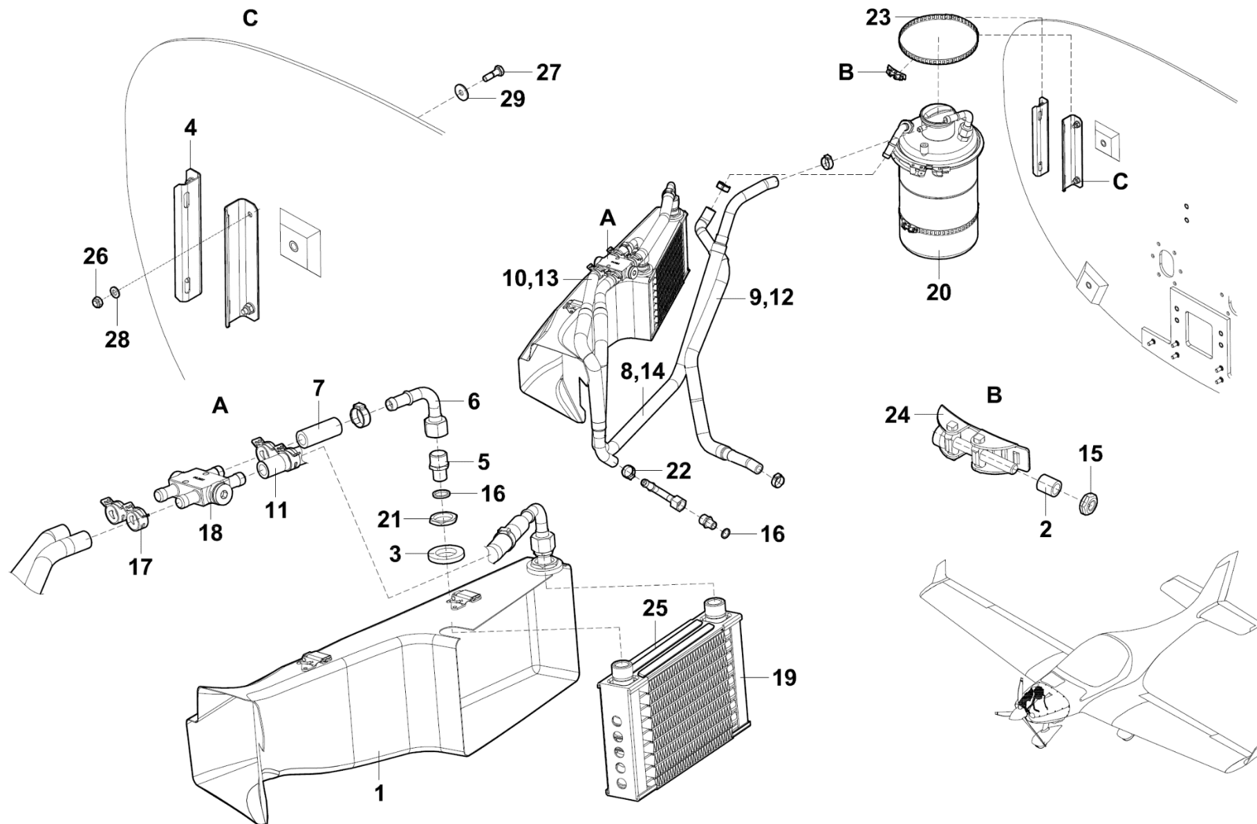
Figure 79-20-01 Oil system LSA
