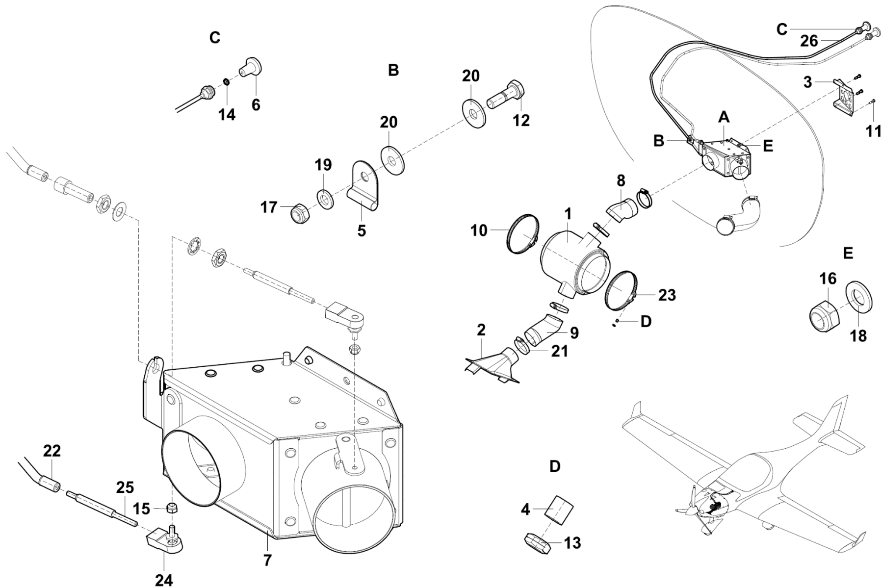
Figure 21-40-01 Heating LSA
