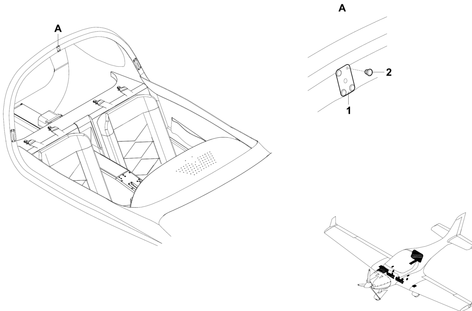
Figure 53-10-02 Fuselage FG LSA
