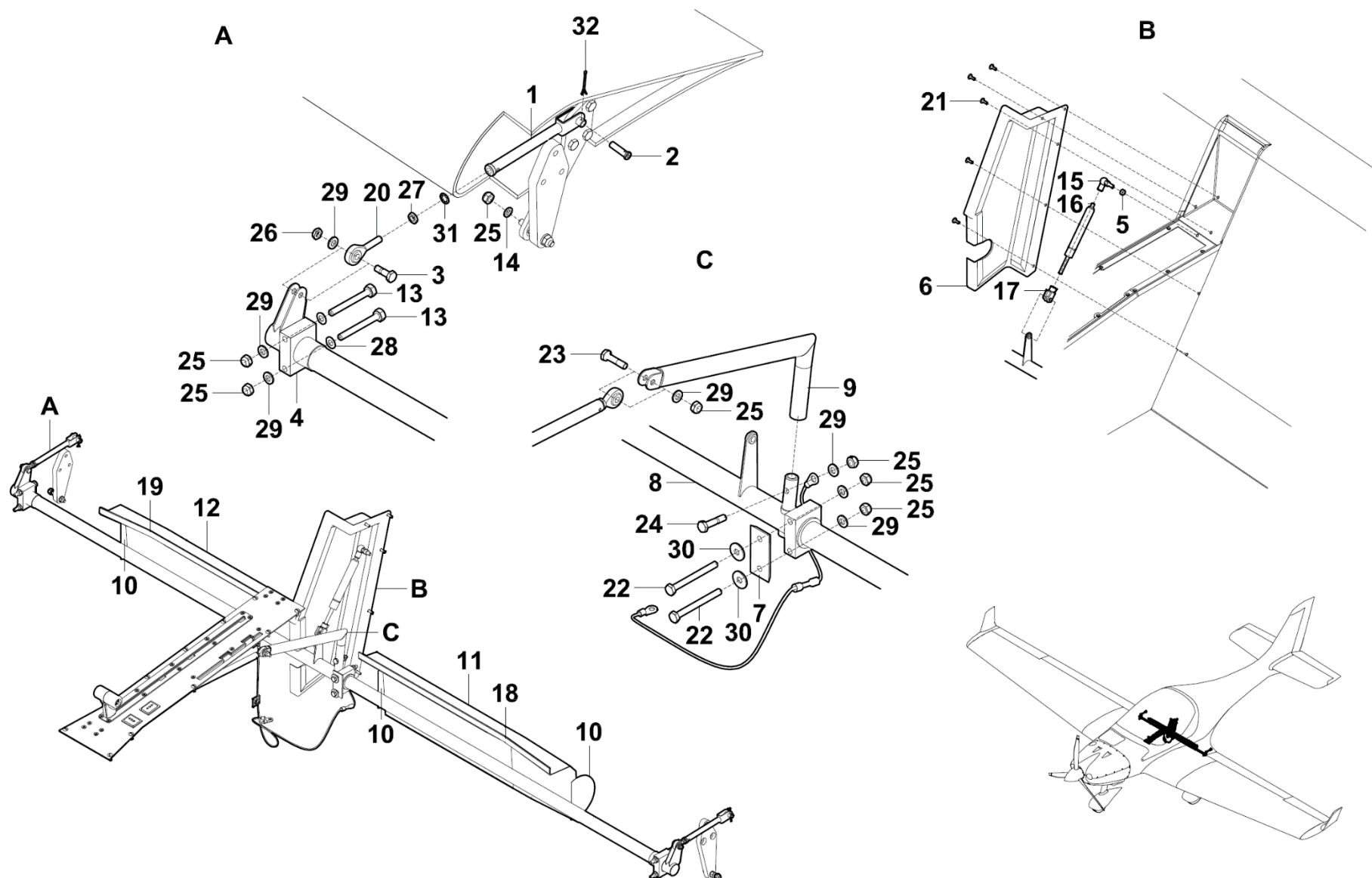
Figure 27-50-01 Flaps Control LSA
