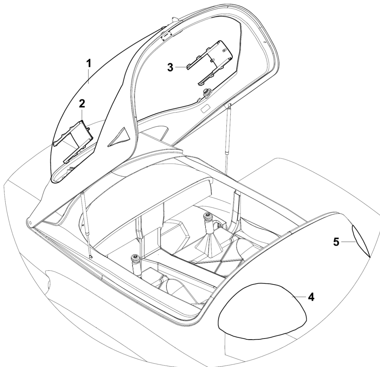
Figure 56-10 Windows LSA
