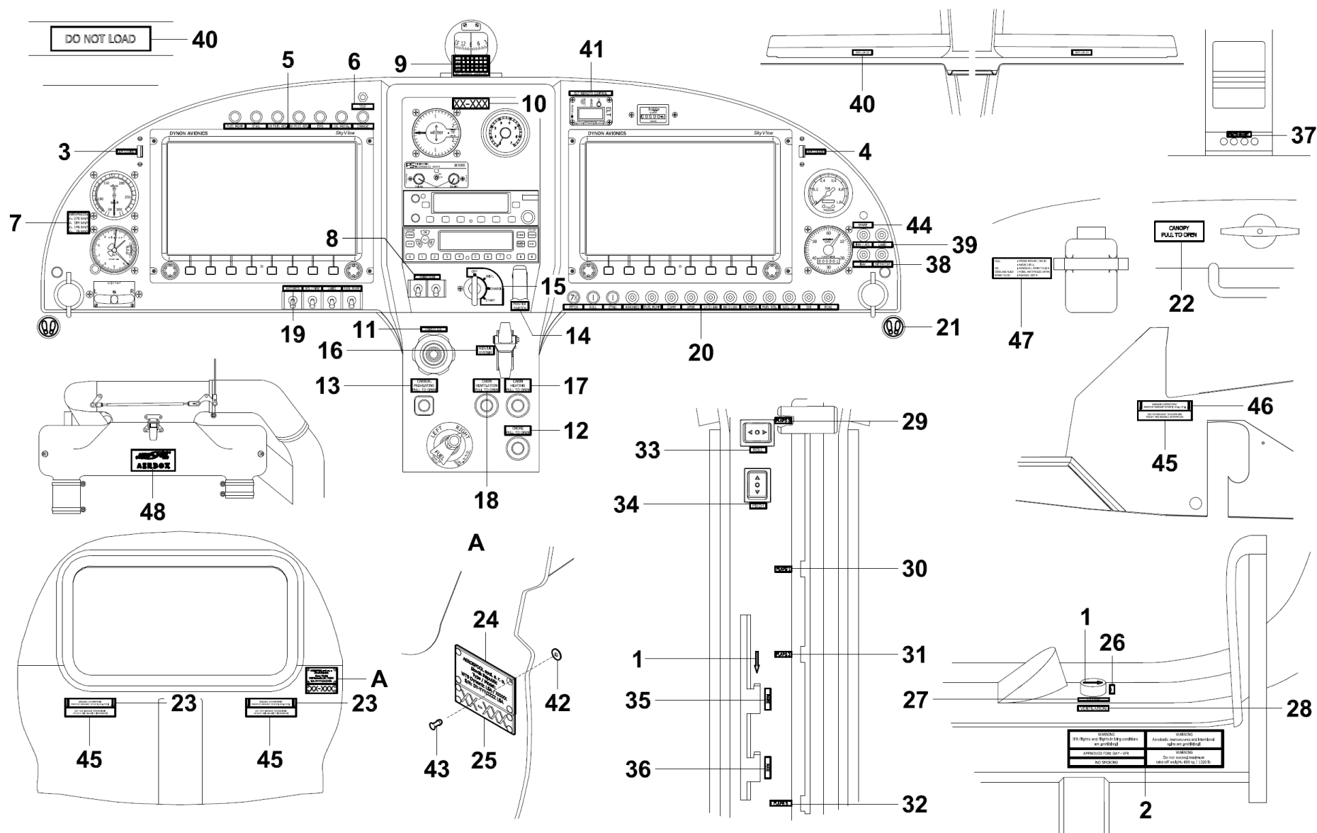
Figure 11-30-01 Placards and labels, Interior
