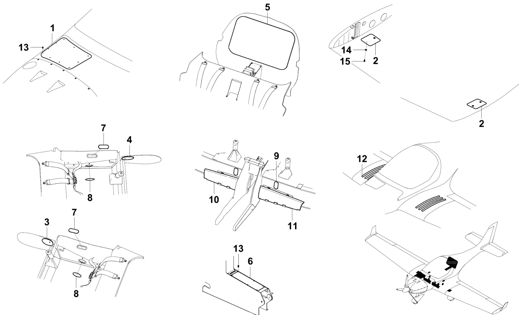
Figure 53-10-01 Fuselage FG LSA
