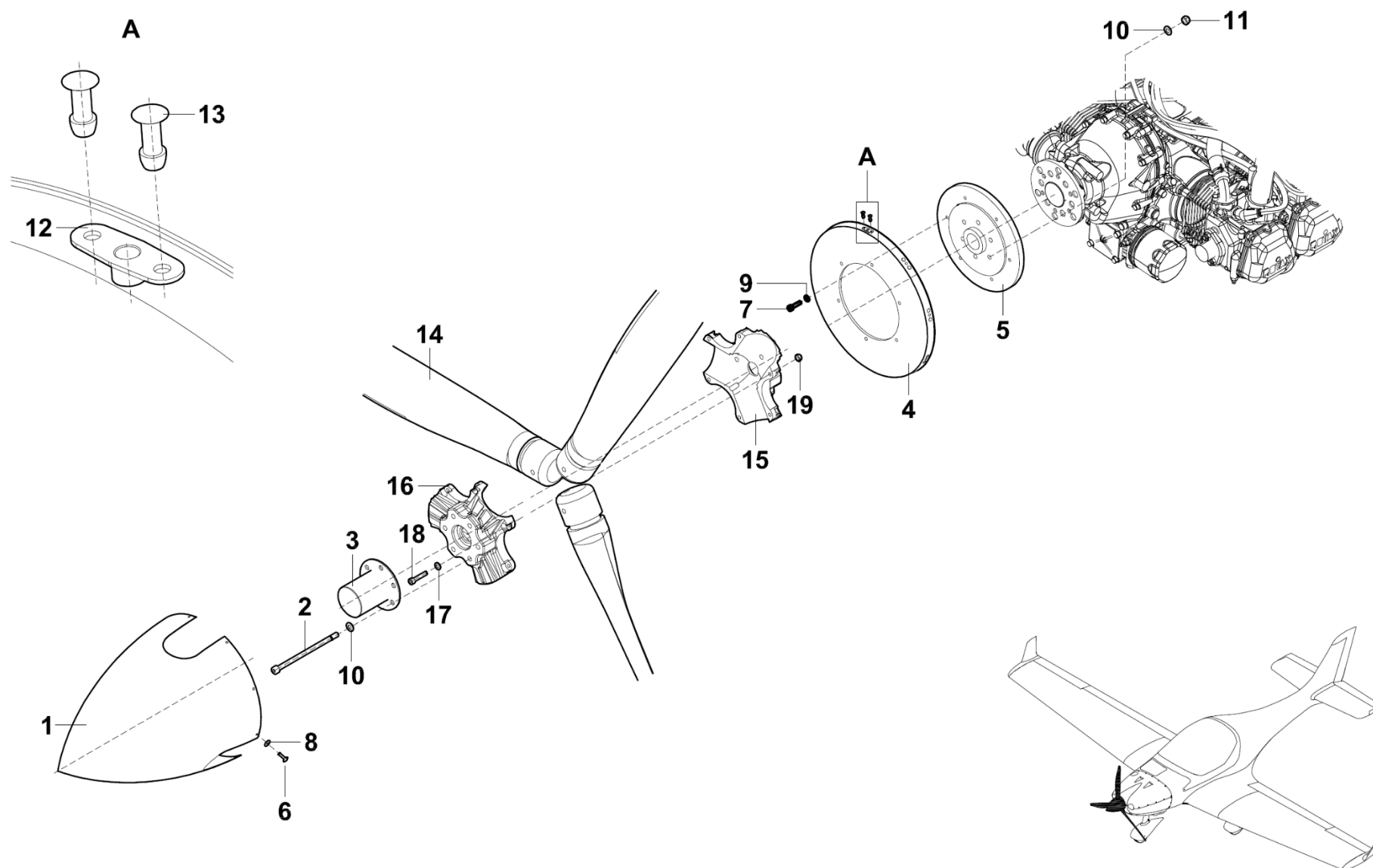
Figure 61-10 Installation of Propeller
