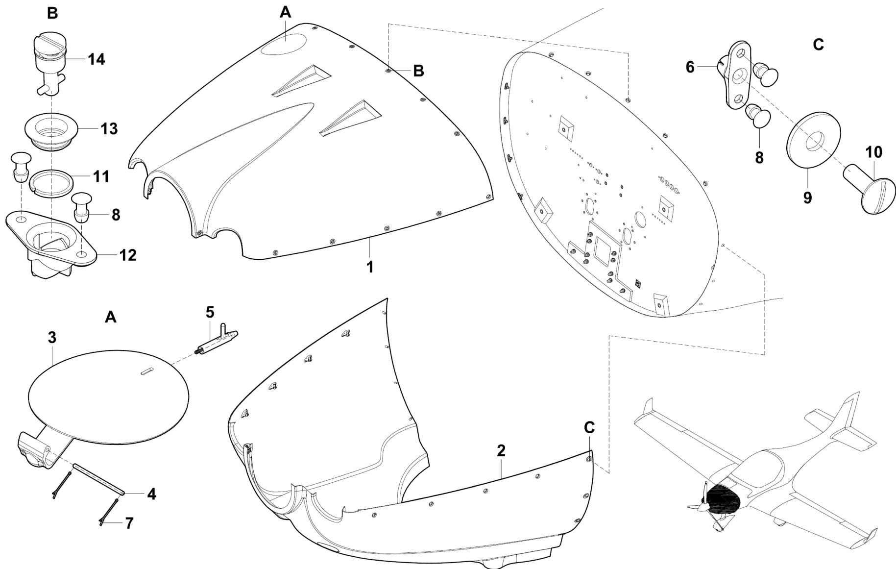
Figure 71-10 Engine Cowlings LSA
