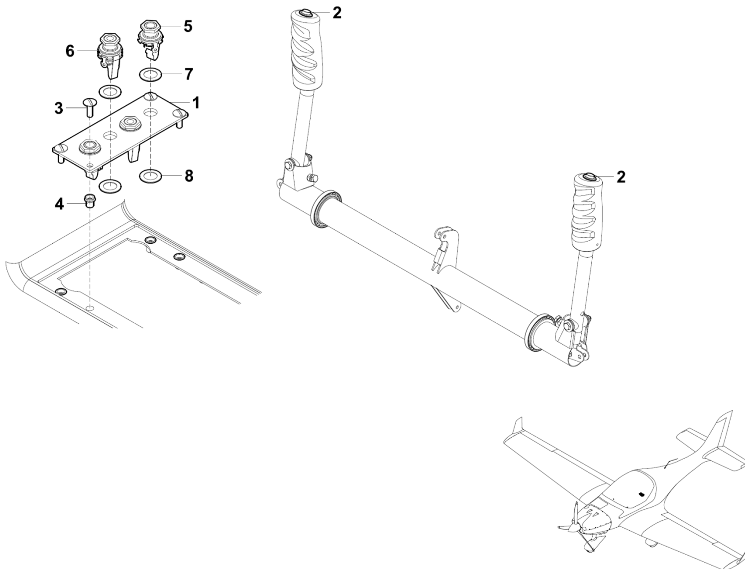
Figure 23-50-01 Audio integrating
