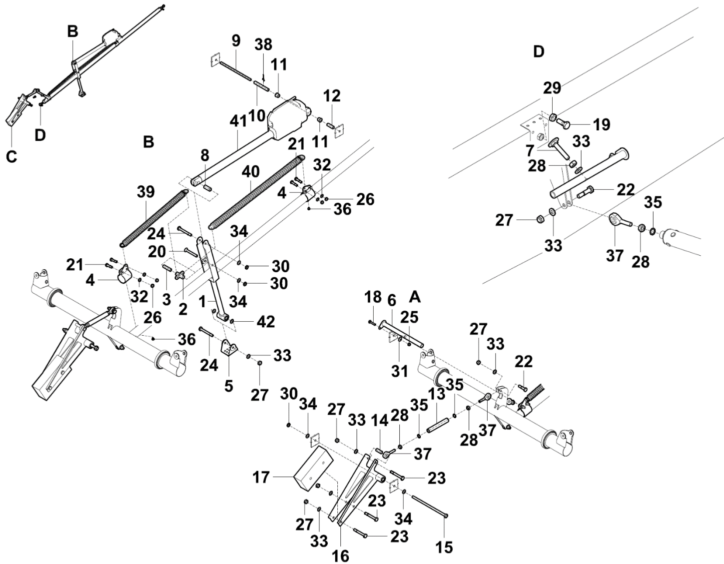
Figure 27-30-02 Elevator Control LSA
