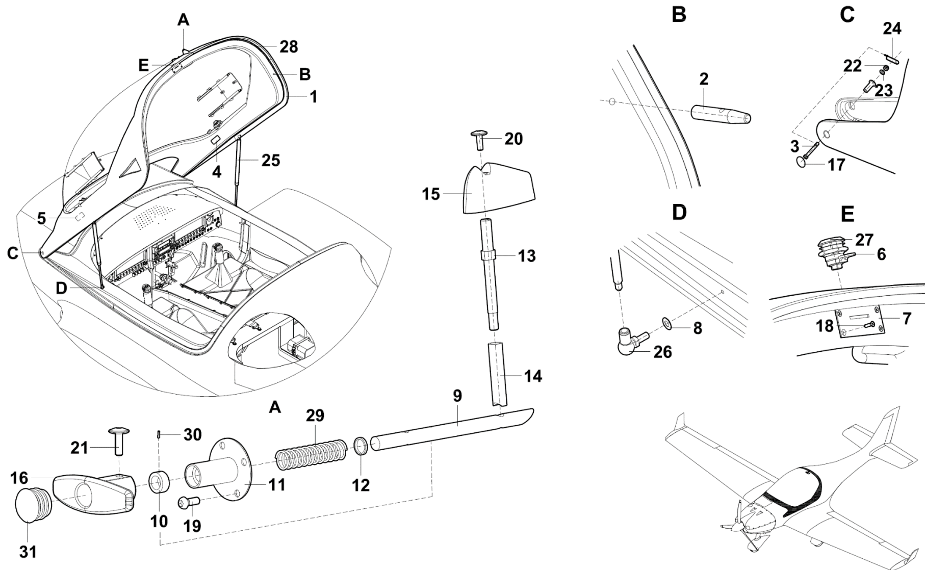
Figure 52-10 Canopy frame LSA
