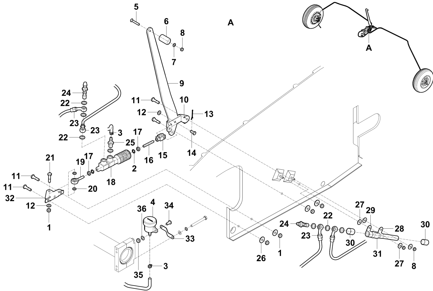
Figure 32-40-02 Wheels and Brakes LSA
