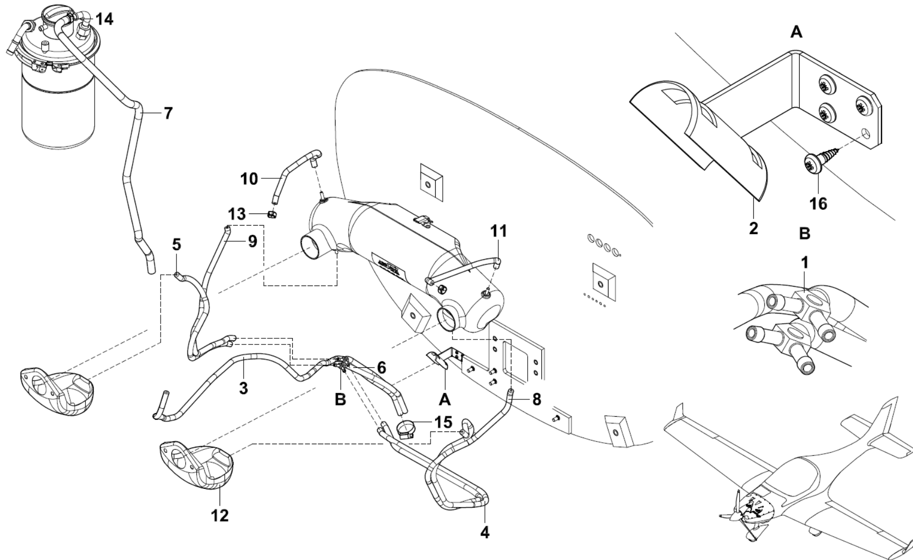
Figure 71-70-01 Engine Drains
