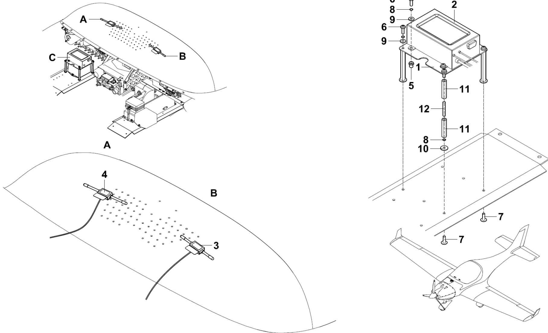
Figure 34-40-01 Independent position determining
