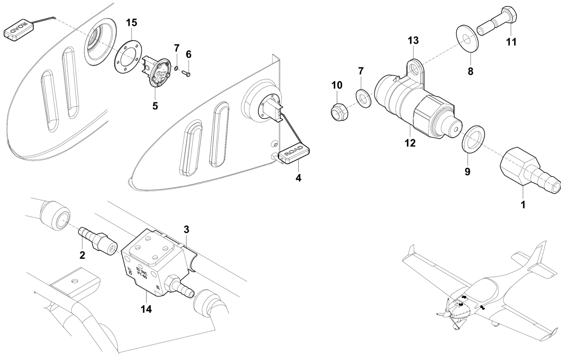
Figure 28-40 Fuel Indicating
