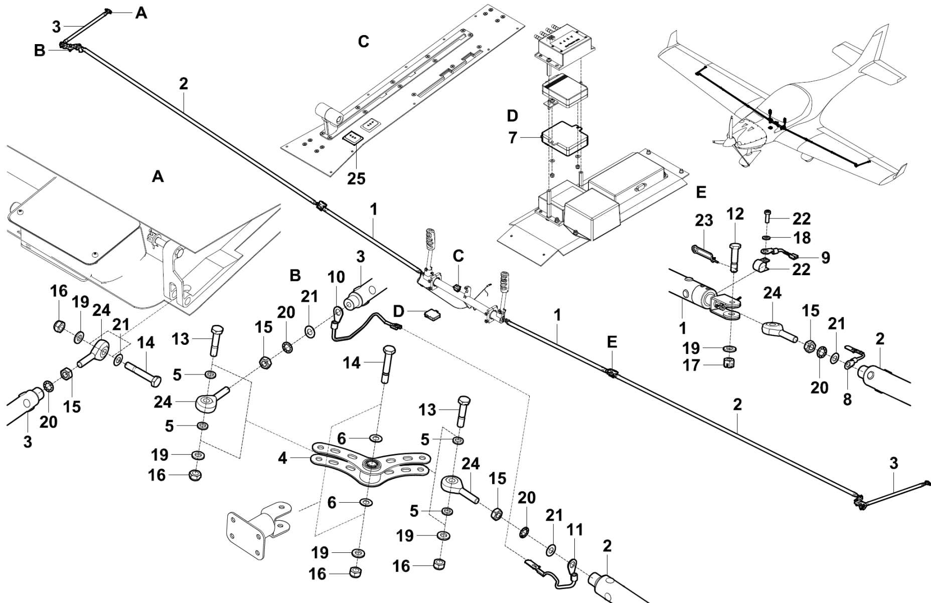
Figure 27-10-01 Aileron Control LSA
