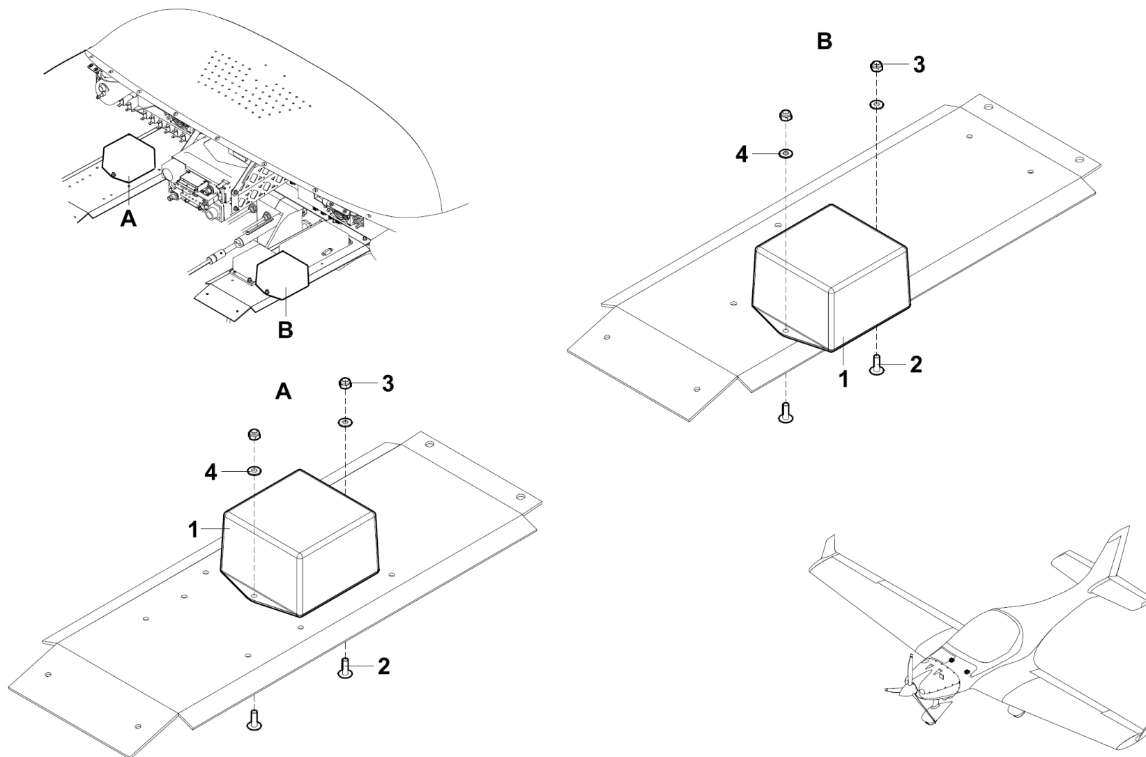
Figure 24-30-02 DC Generation LSA
