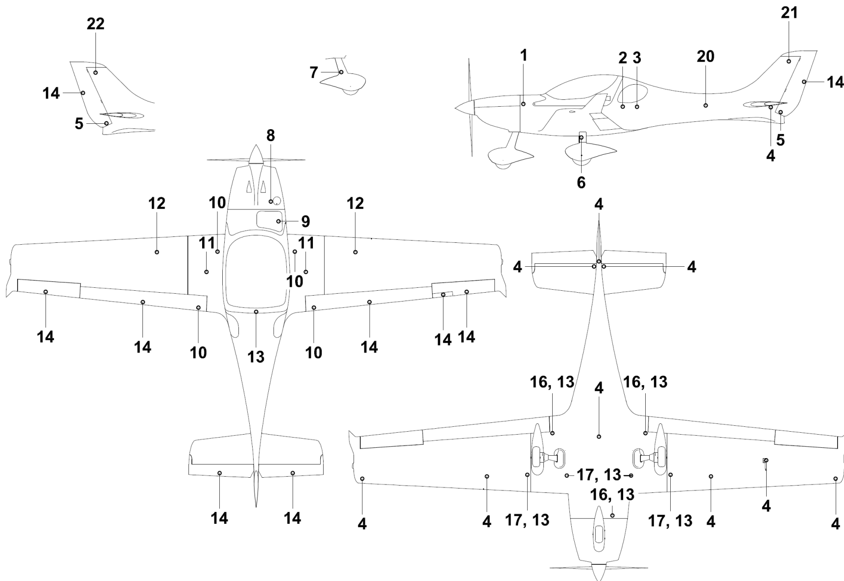
Figure 11-20-01 Placards and labels, Exterior
