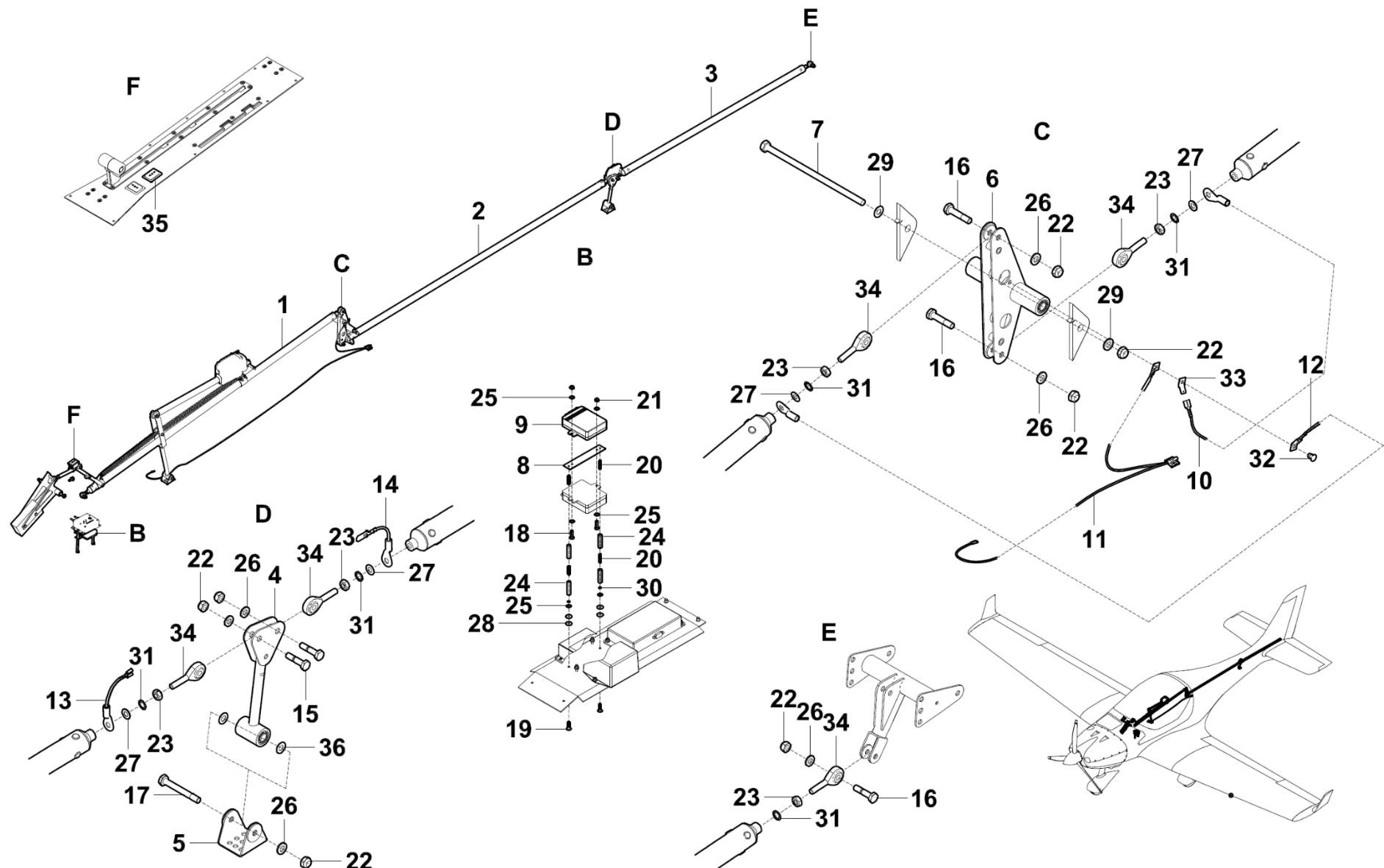
Figure 27-30-01 Elevator Control LSA
