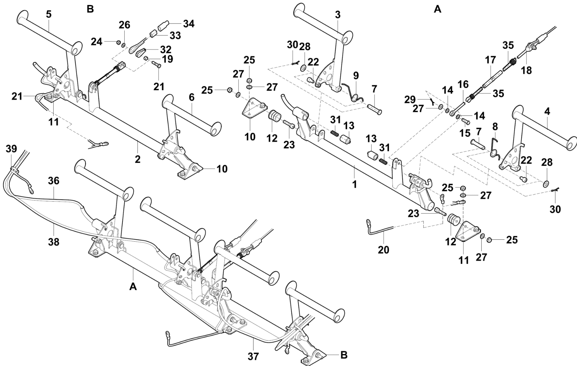
Figure 27-20-02 Rudder Control LSA
