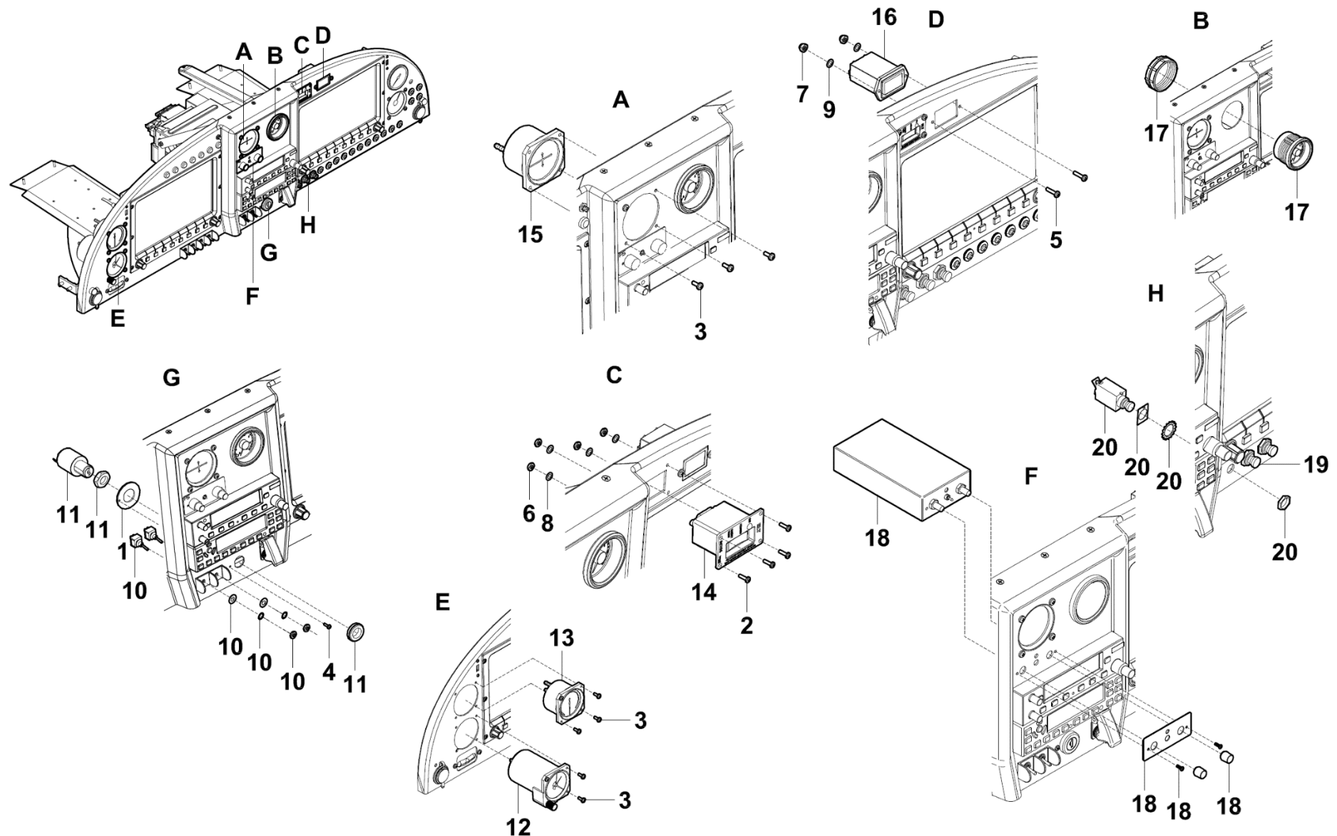
Figure 39-10-03 Instrument Panel Installation
