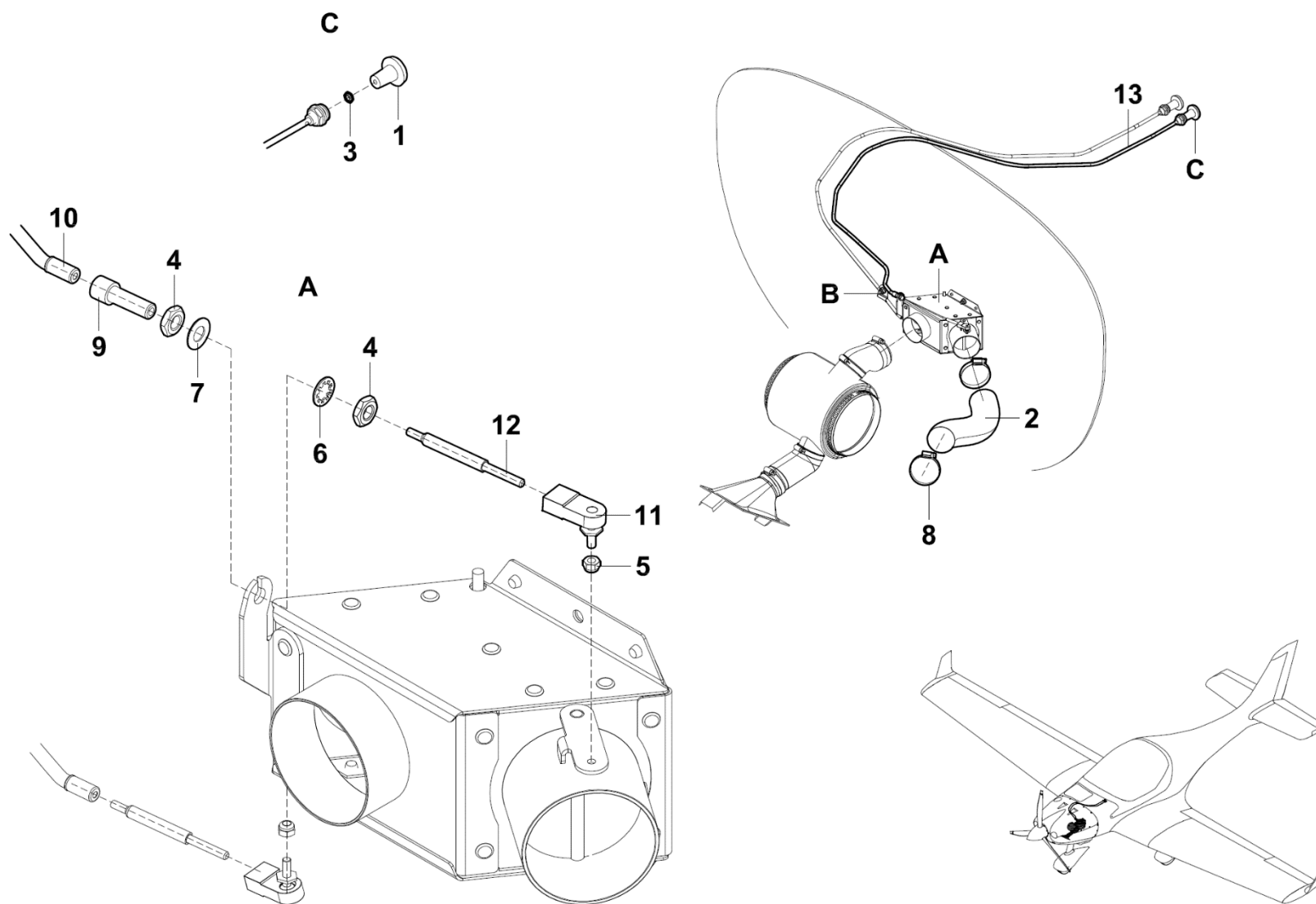
Figure 21-20-01 Venting LSA
