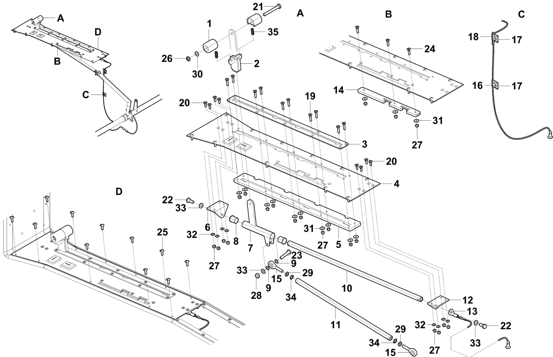
Figure 27-50-02 Flaps Control LSA
