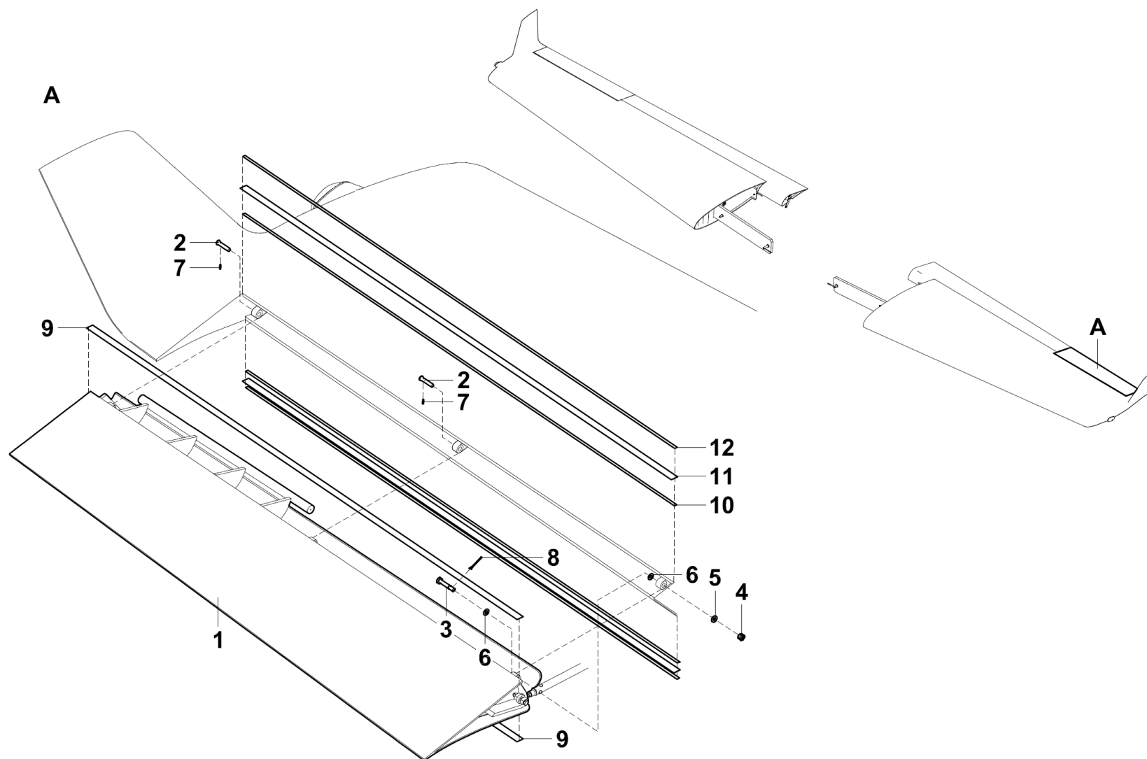
Figure 57-60-02 Ailerons LSA
