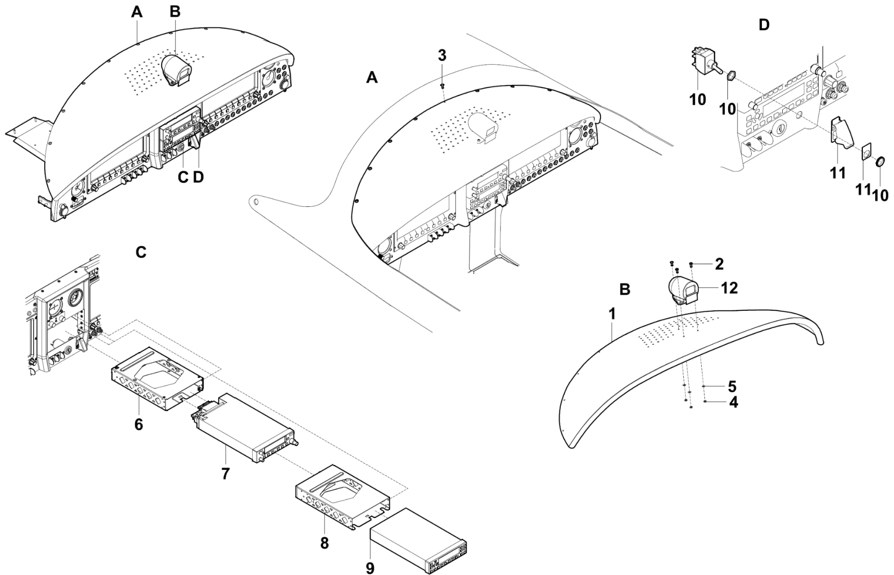
Figure 39-10-05 Instrument Panel Installation
