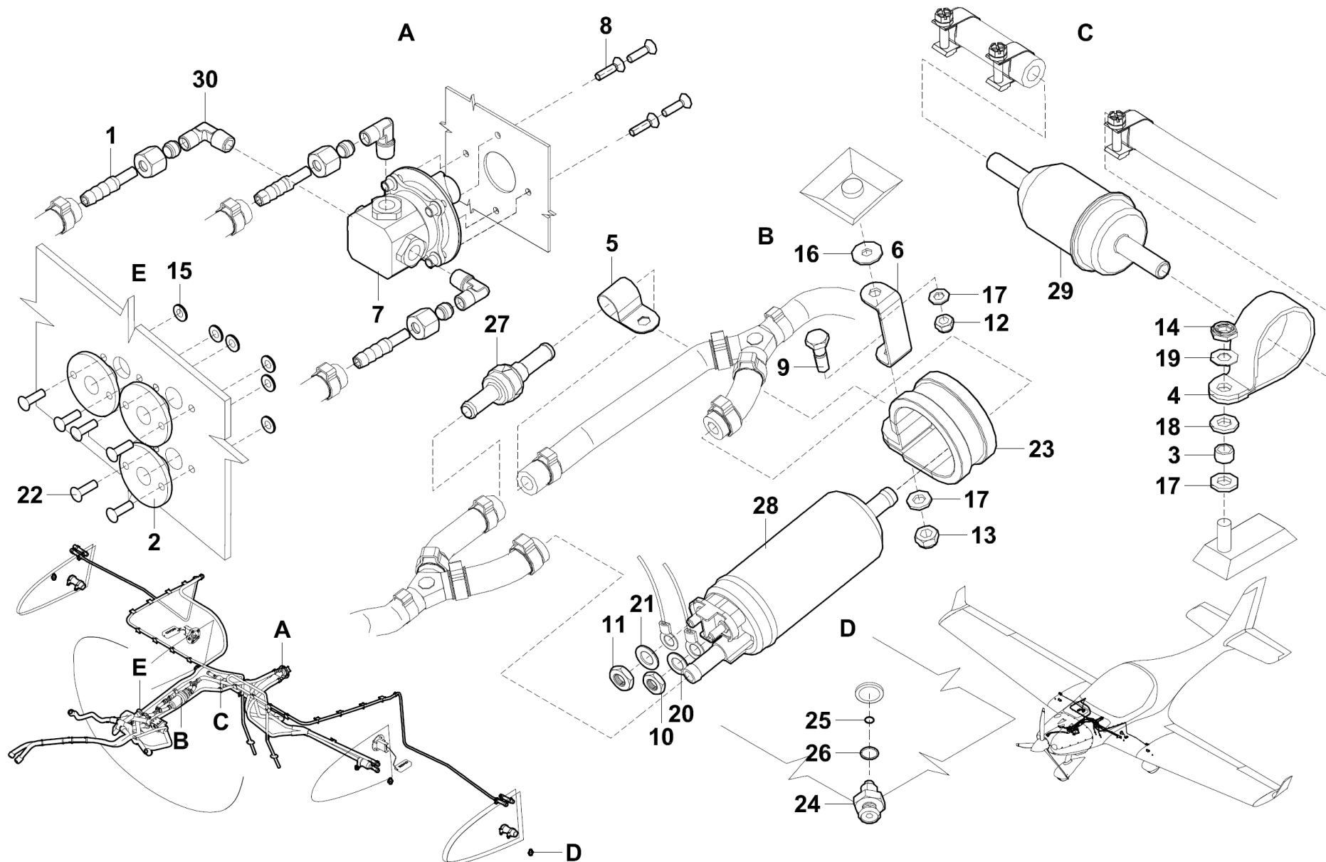
Figure 28-20-01 Fuel System LSA
