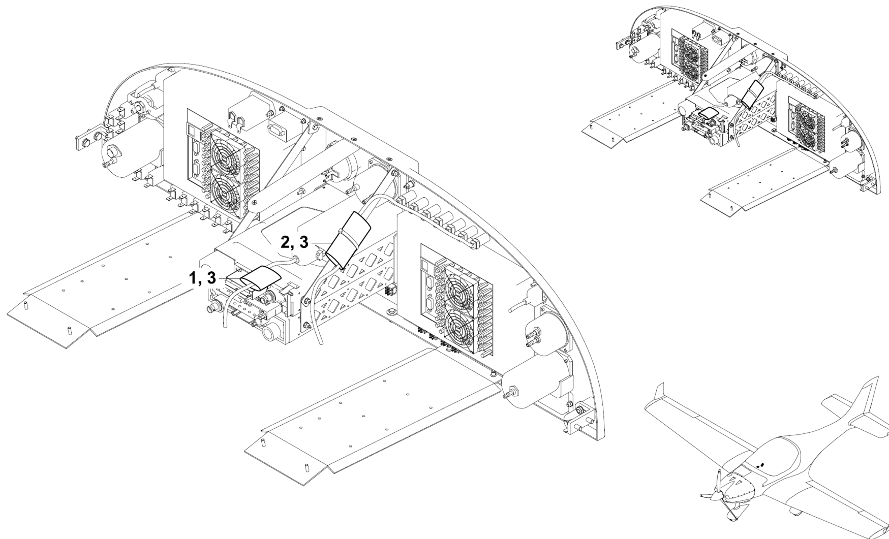
Figure 39-30-01 Electric Junction Boxes
