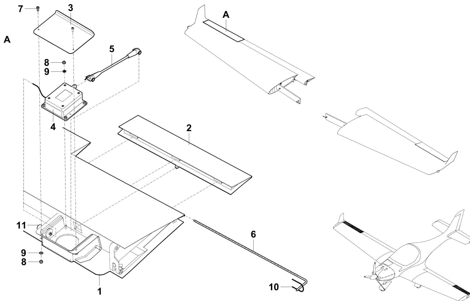
Figure 57-60-01 Ailerons LSA
