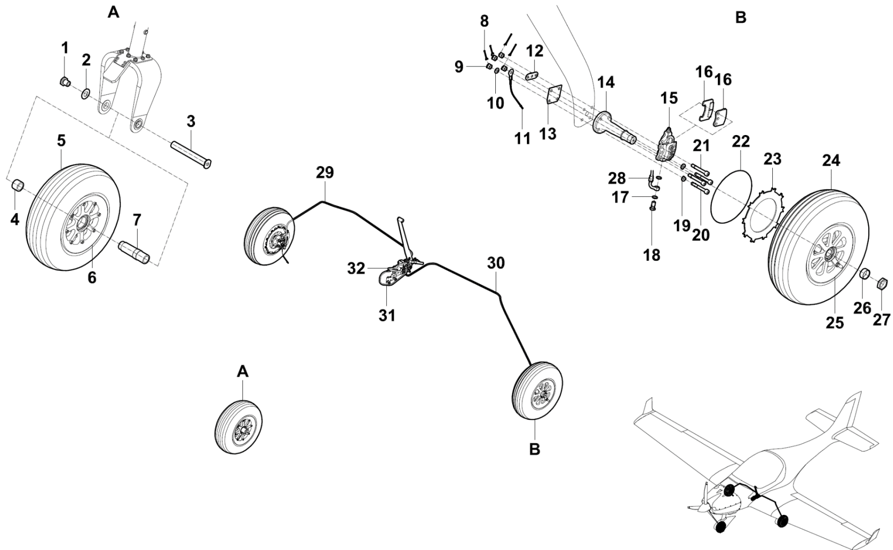
Figure 32-40-01 Wheels and Brakes LSA
