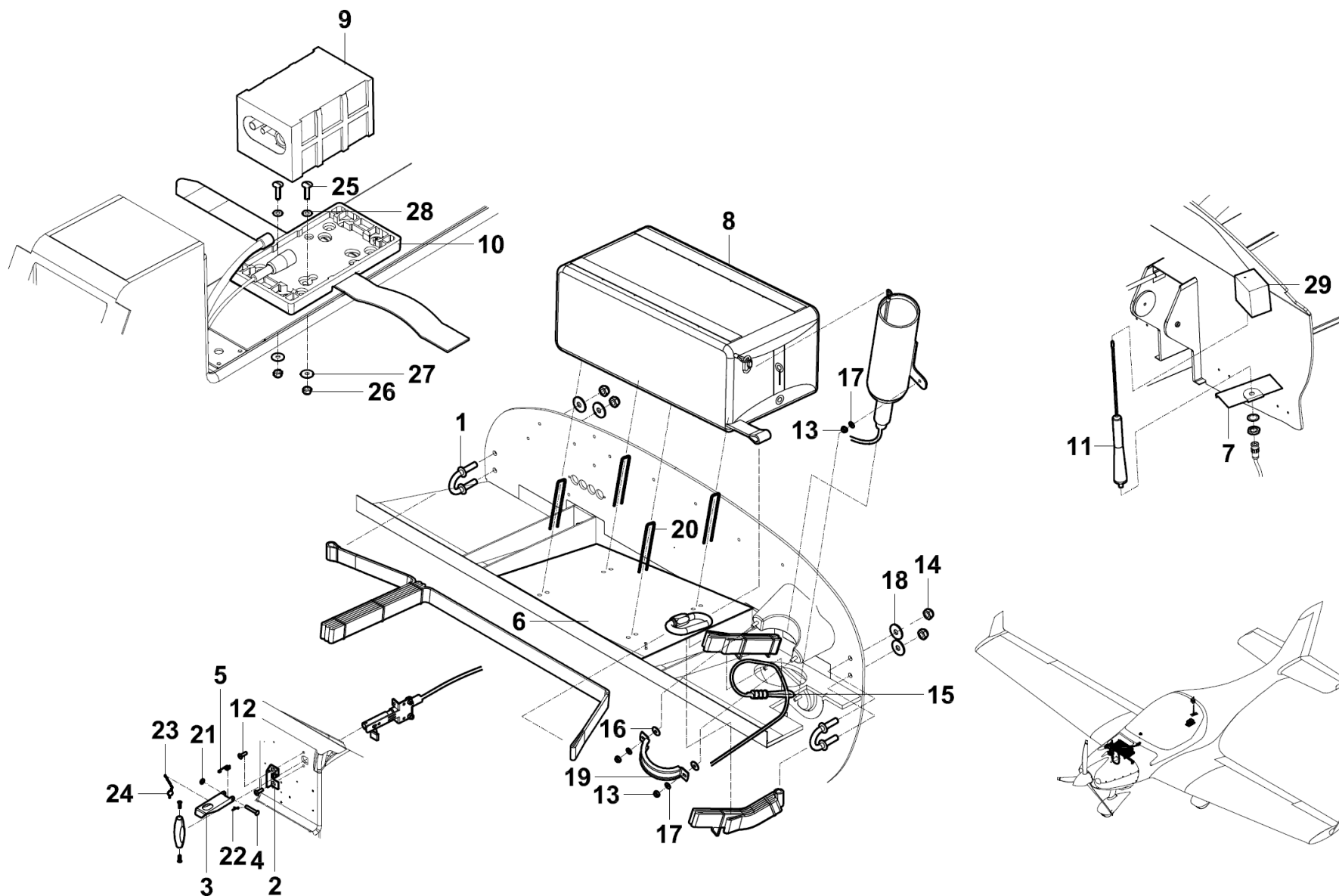
Figure 25-60-01 Emergency systems LSA
