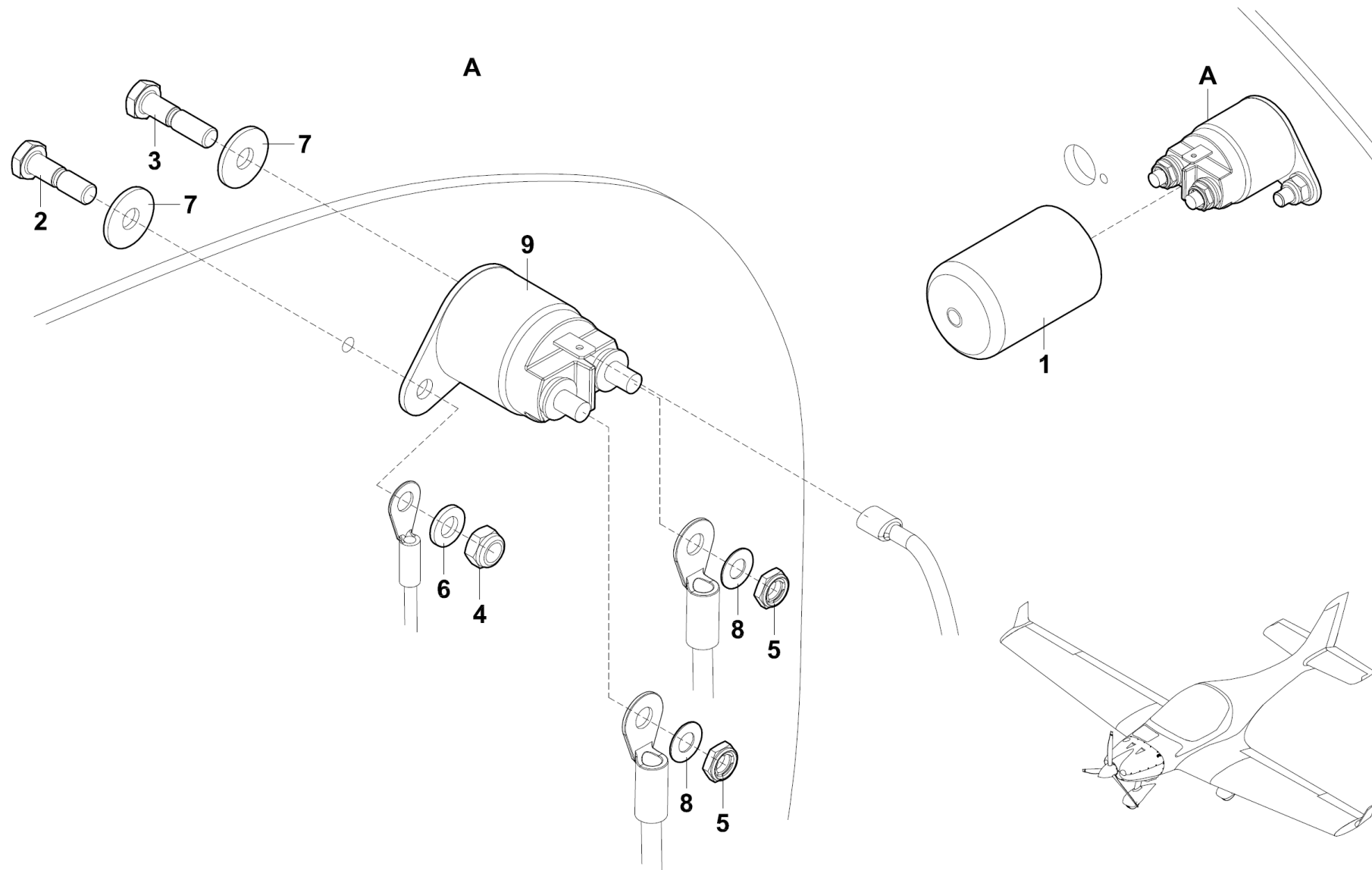
Figure 24-60-02 DC Distribution LSA
