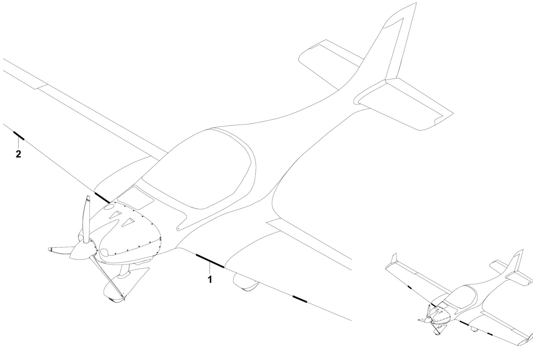
Figure 57-40 Stallstrips LSA
