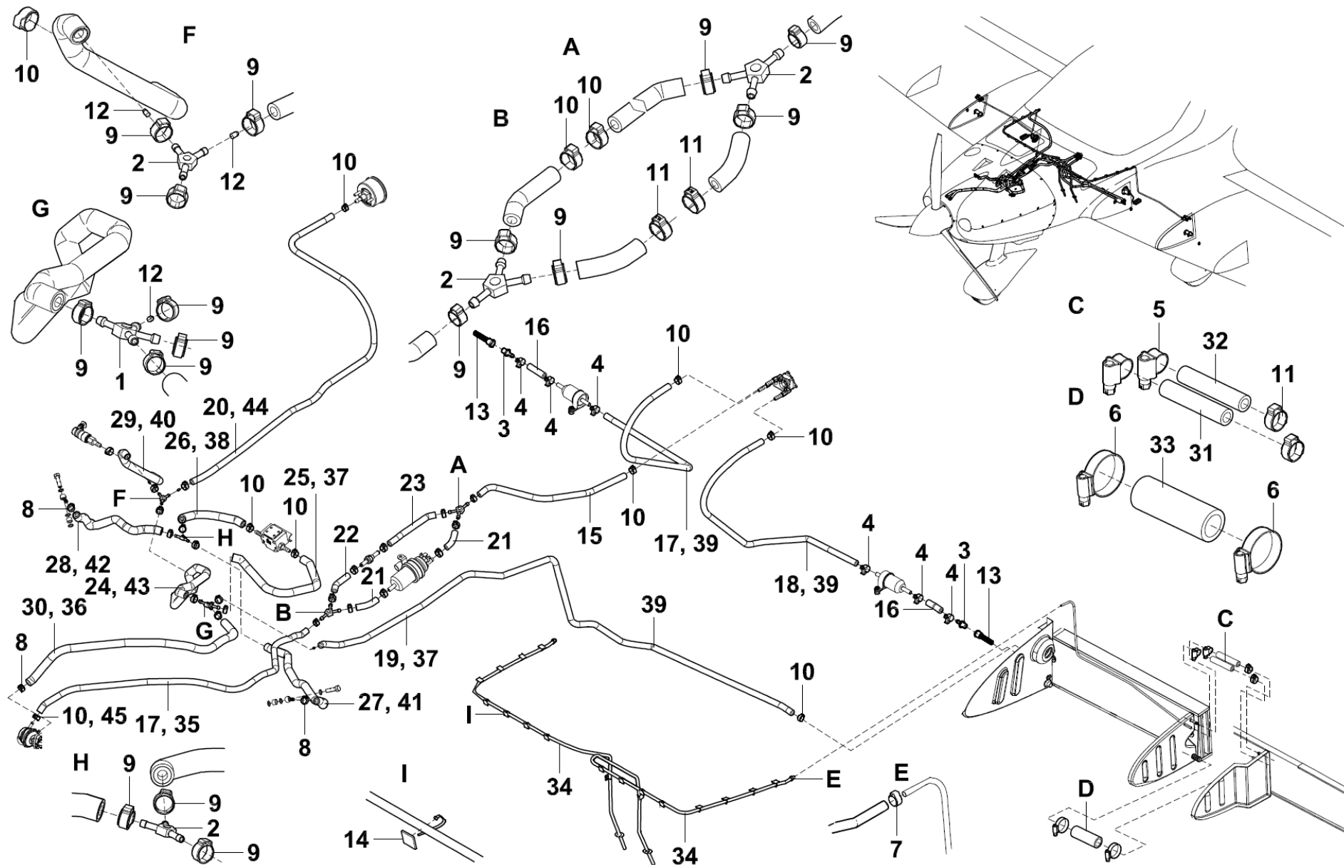
Figure 28-20-02 Fuel System LSA
